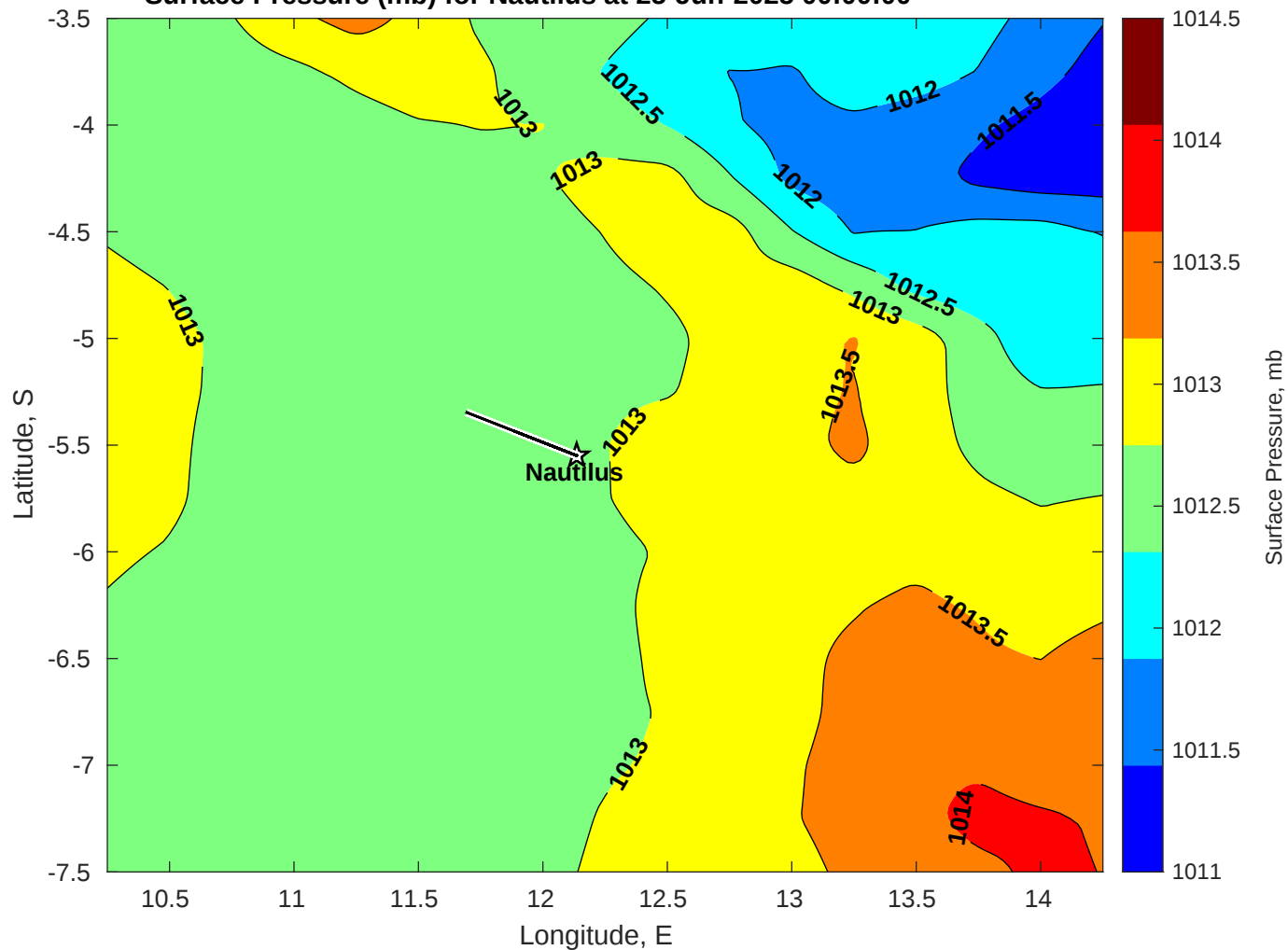
Surface Pressure (mb) for Nautilus at 25-Jun-2025 00:00:00
