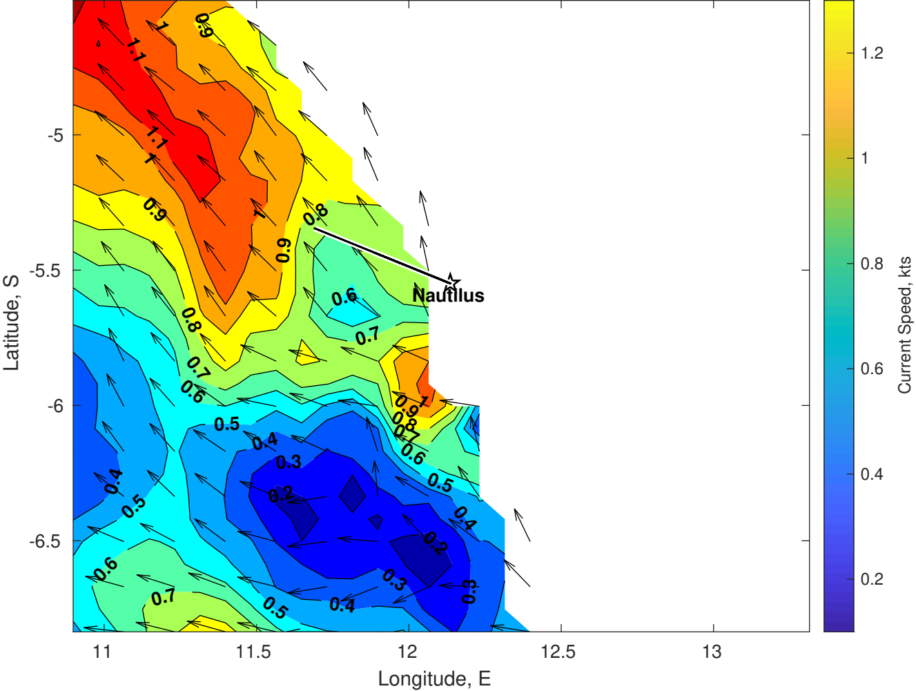
Surface Currents for Nautilus at 22-Jun-2025 00:00:00
