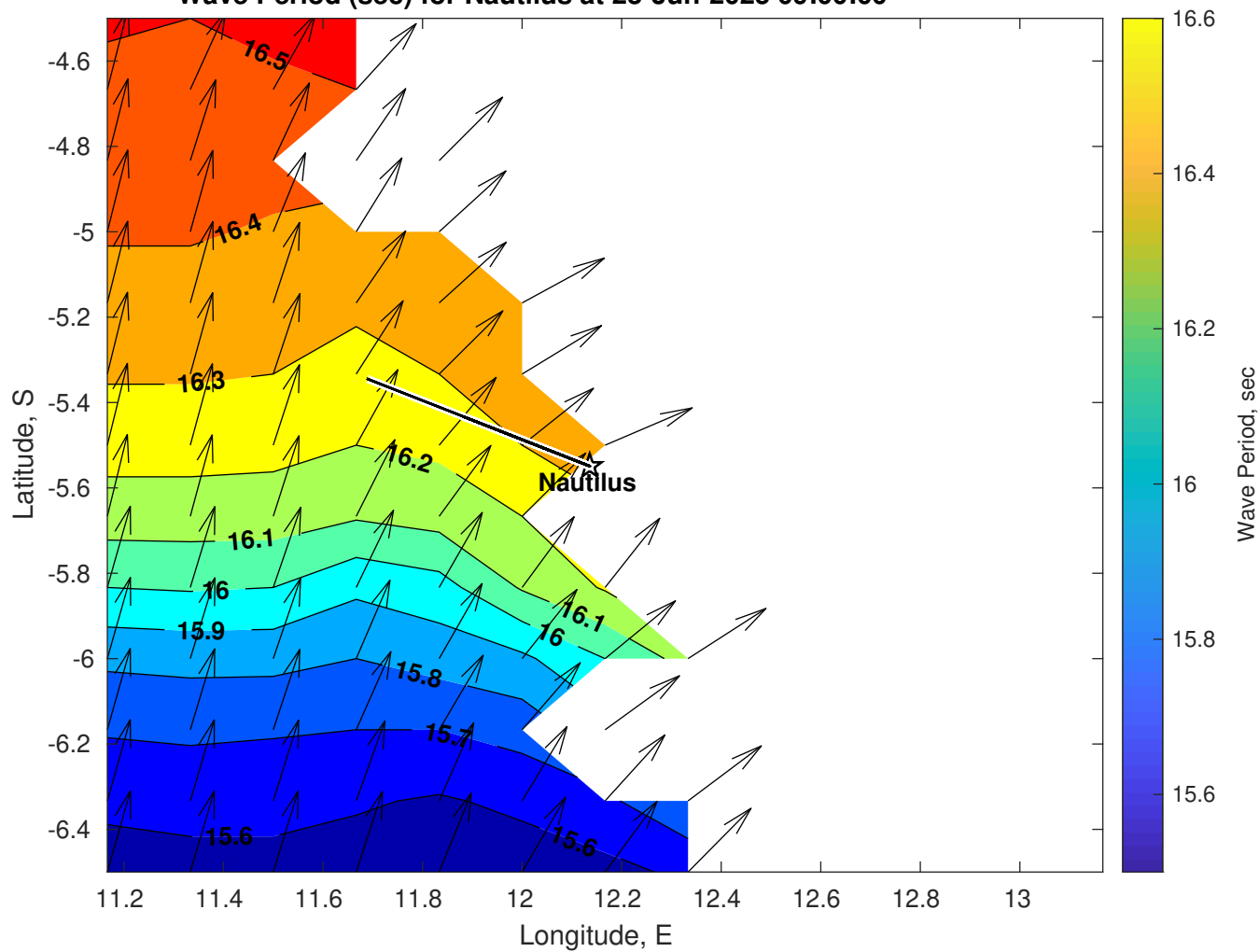
Wave Period (sec) for Nautilus at 23-Jun-2025 09:00:00
