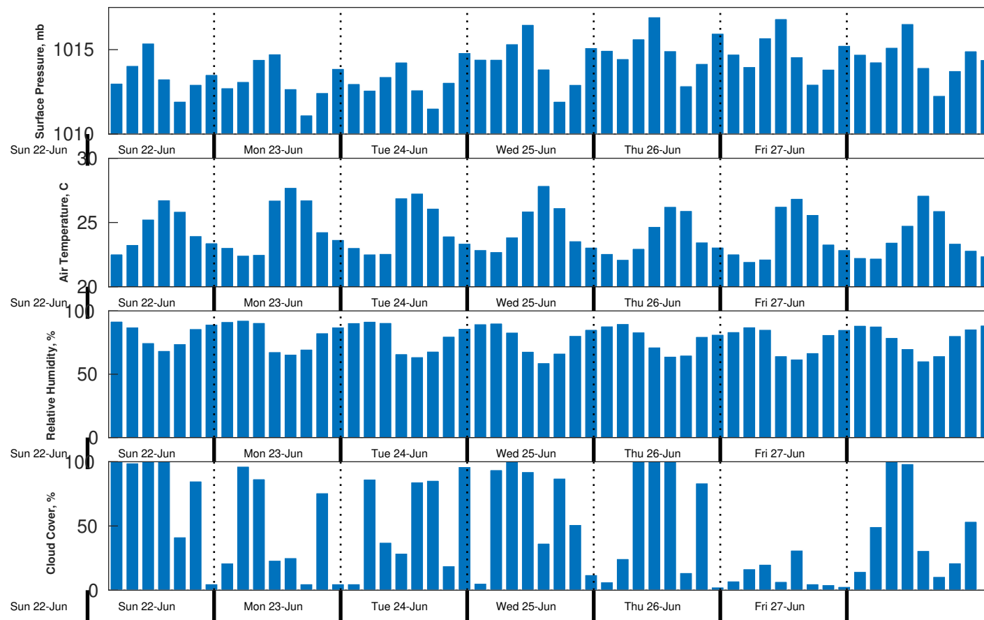
Met Forecast for Nautilus from 23-Jun-2025 00:00:00 to 30-Jun-2025 00:00:00
