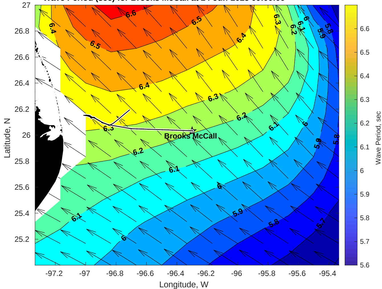
Wave Period (sec) for Brooks McCall at 24-Jun-2025 09:00:00
