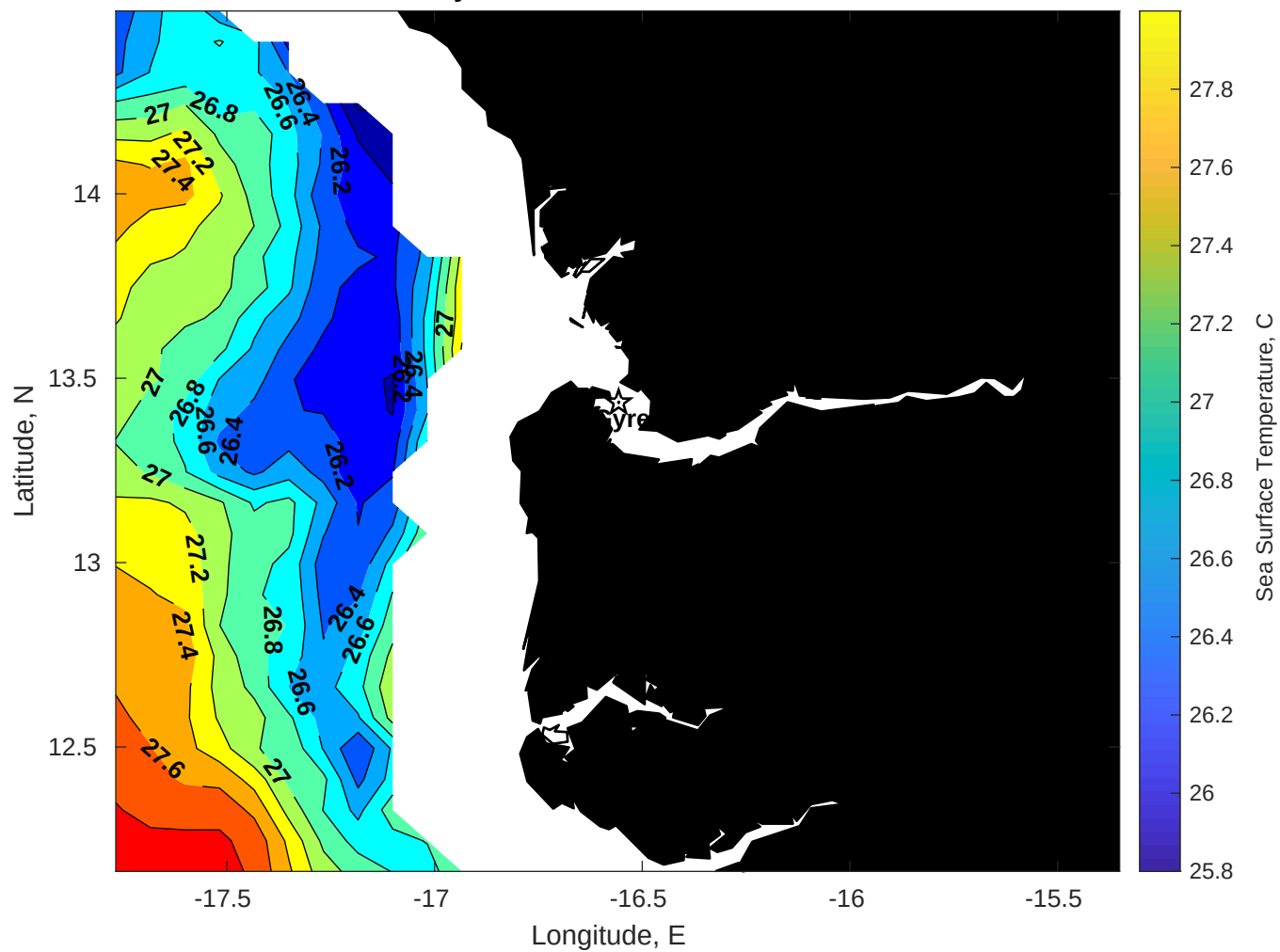
SST for Gyre at 23-Jun-2025 00:00:00
