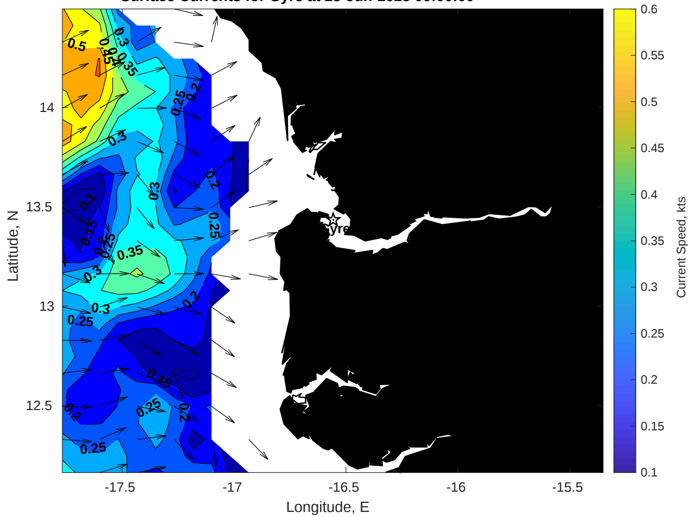
Surface Currents for Gyre at 23-Jun-2025 00:00:00
