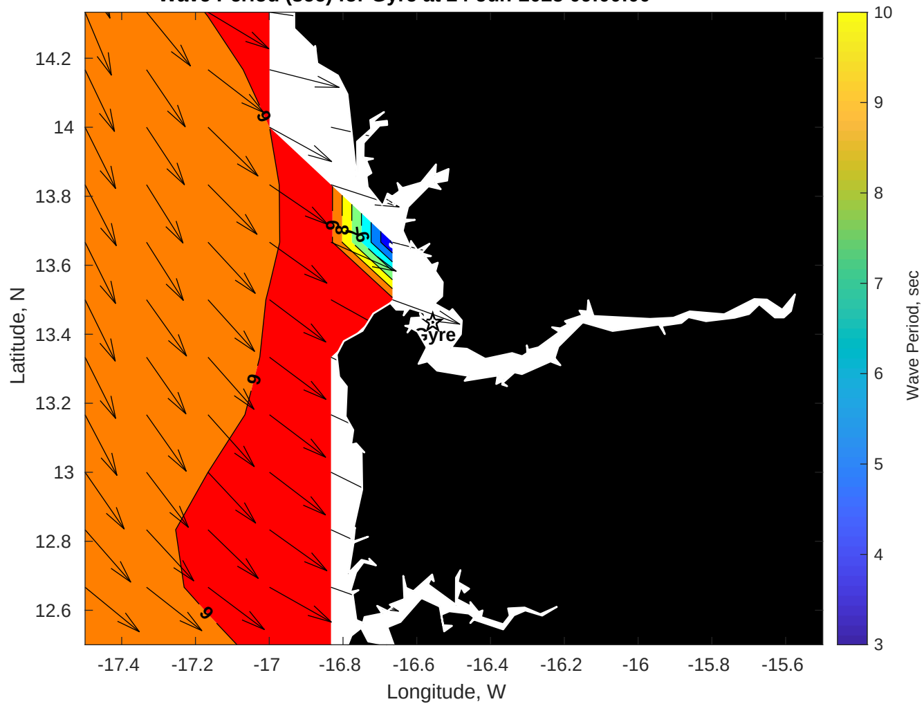
Wave Period (sec) for Gyre at 24-Jun-2025 09:00:00
