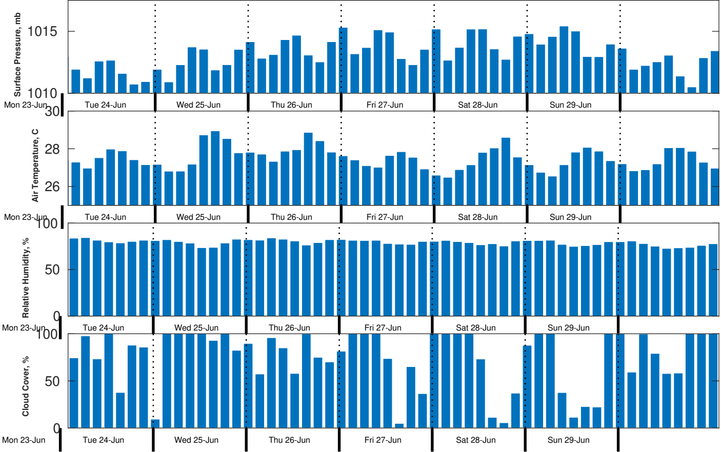
Met Forecast for Gyre from 23-Jun-2025 23:00:00 to 30-Jun-2025 23:00:00
