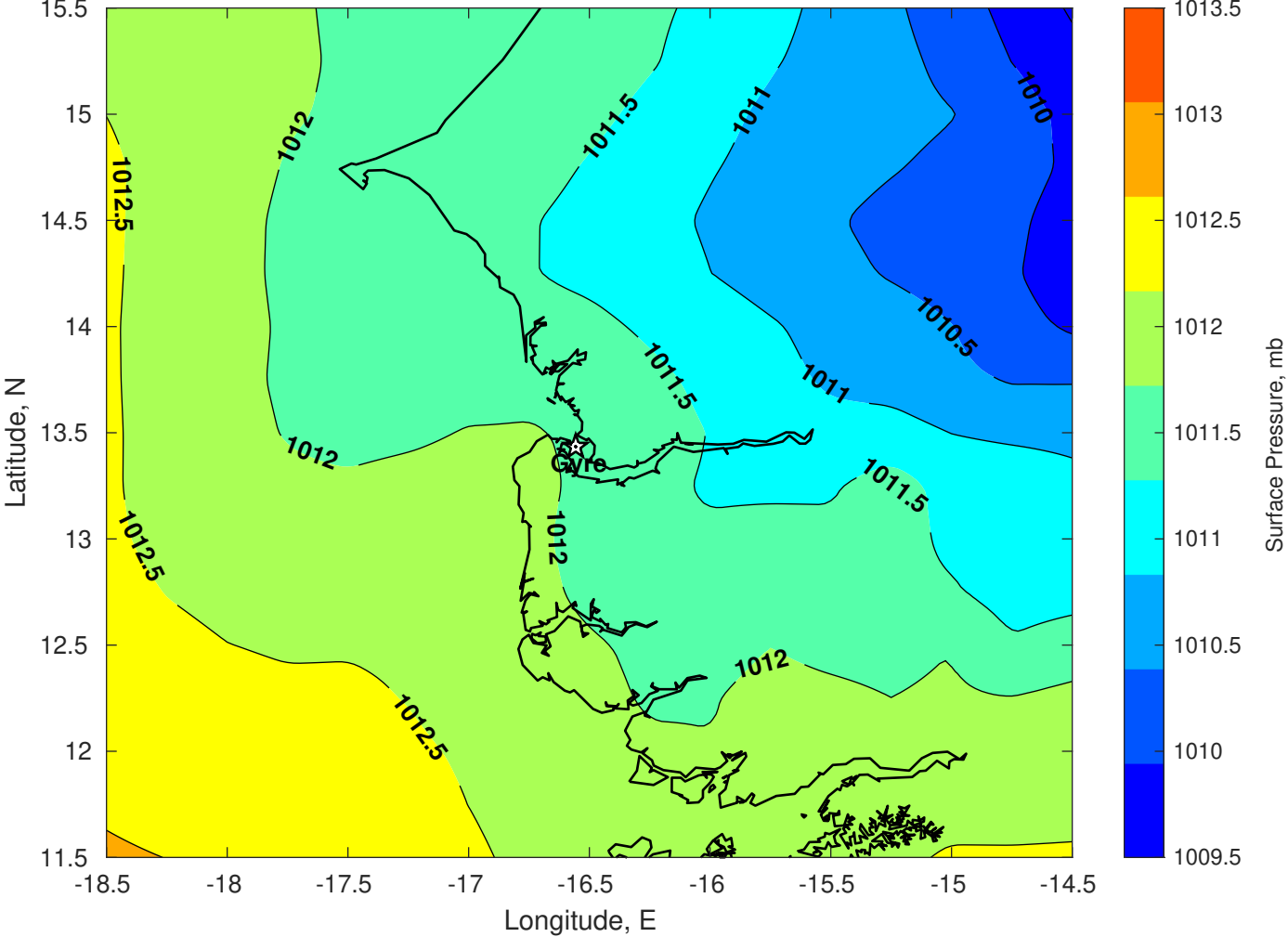
Surface Pressure (mb) for Gyre at 25-Jun-2025 00:00:00
