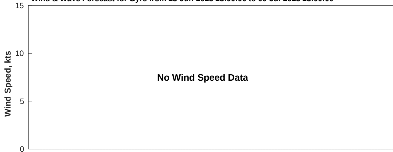
Wind & Wave Forecast for Gyre from 23-Jun-2025 23:00:00 to 09-Jul-2025 23:00:00
