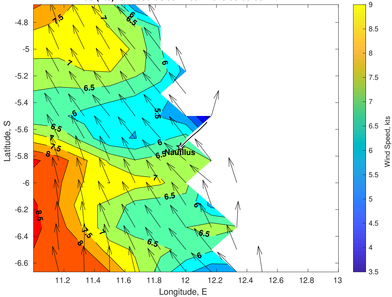
Winds (kts) for Nautilus at 24-Jun-2025 09:00:00
