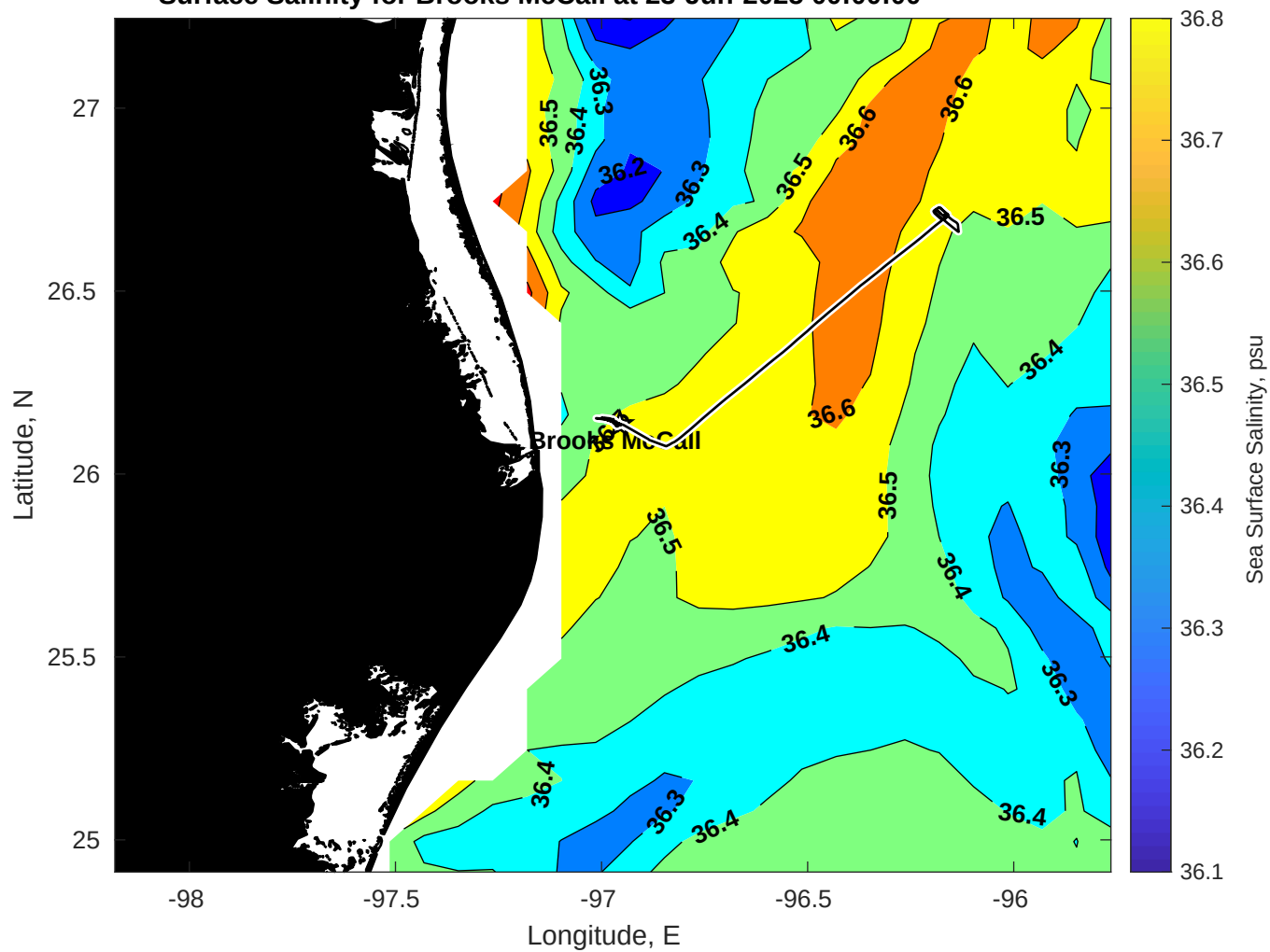
Surface Salinity for Brooks McCall at 23-Jun-2025 00:00:00
