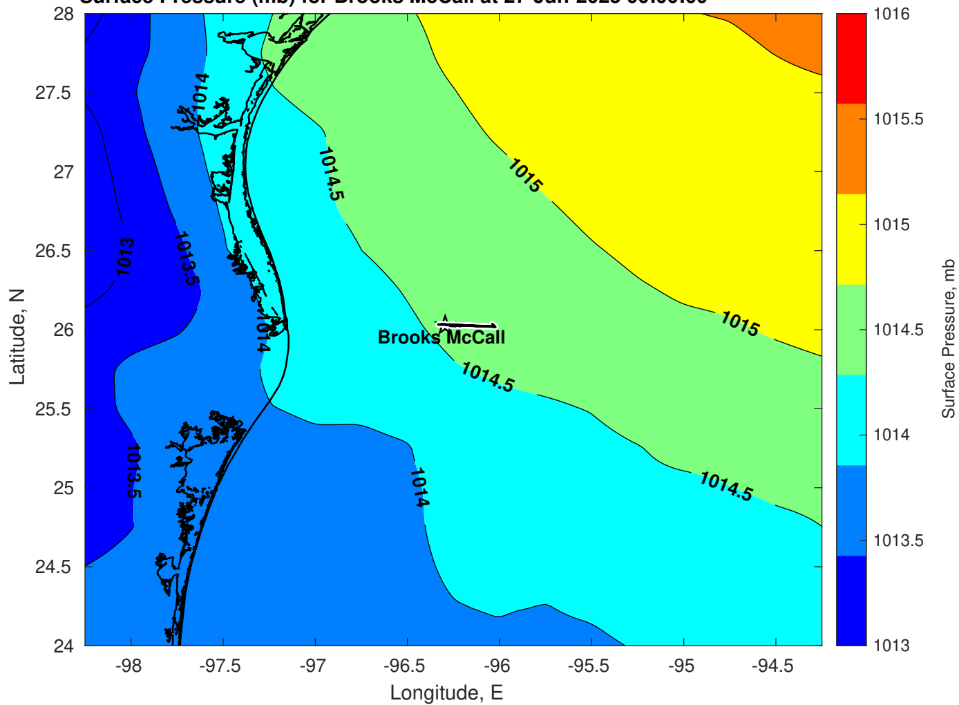
Surface Pressure (mb) for Brooks McCall at 27-Jun-2025 00:00:00
