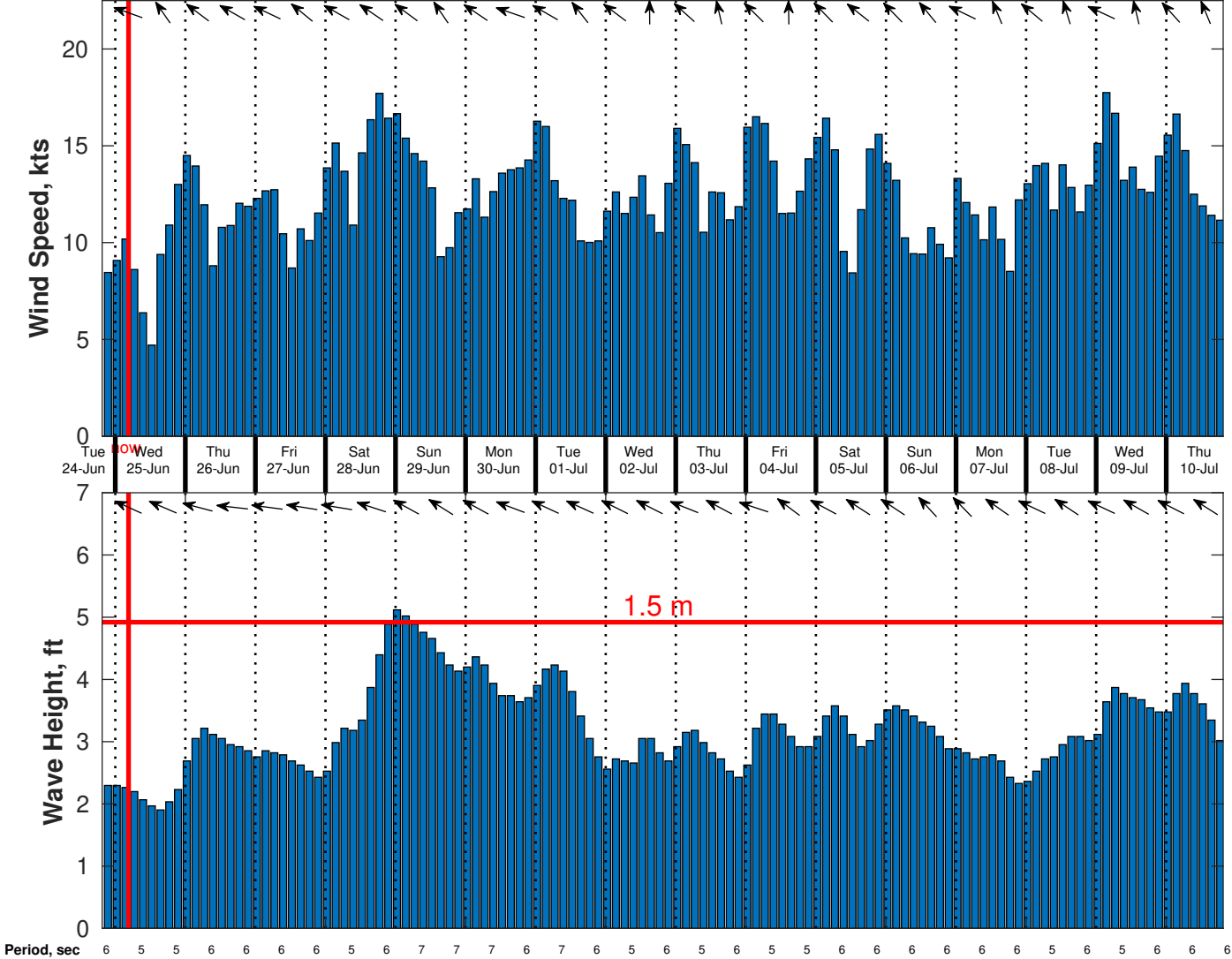
Wind & Wave Forecast for Brooks McCall from 24-Jun-2025 20:00:00 to 10-Jul-2025 20:00:00
