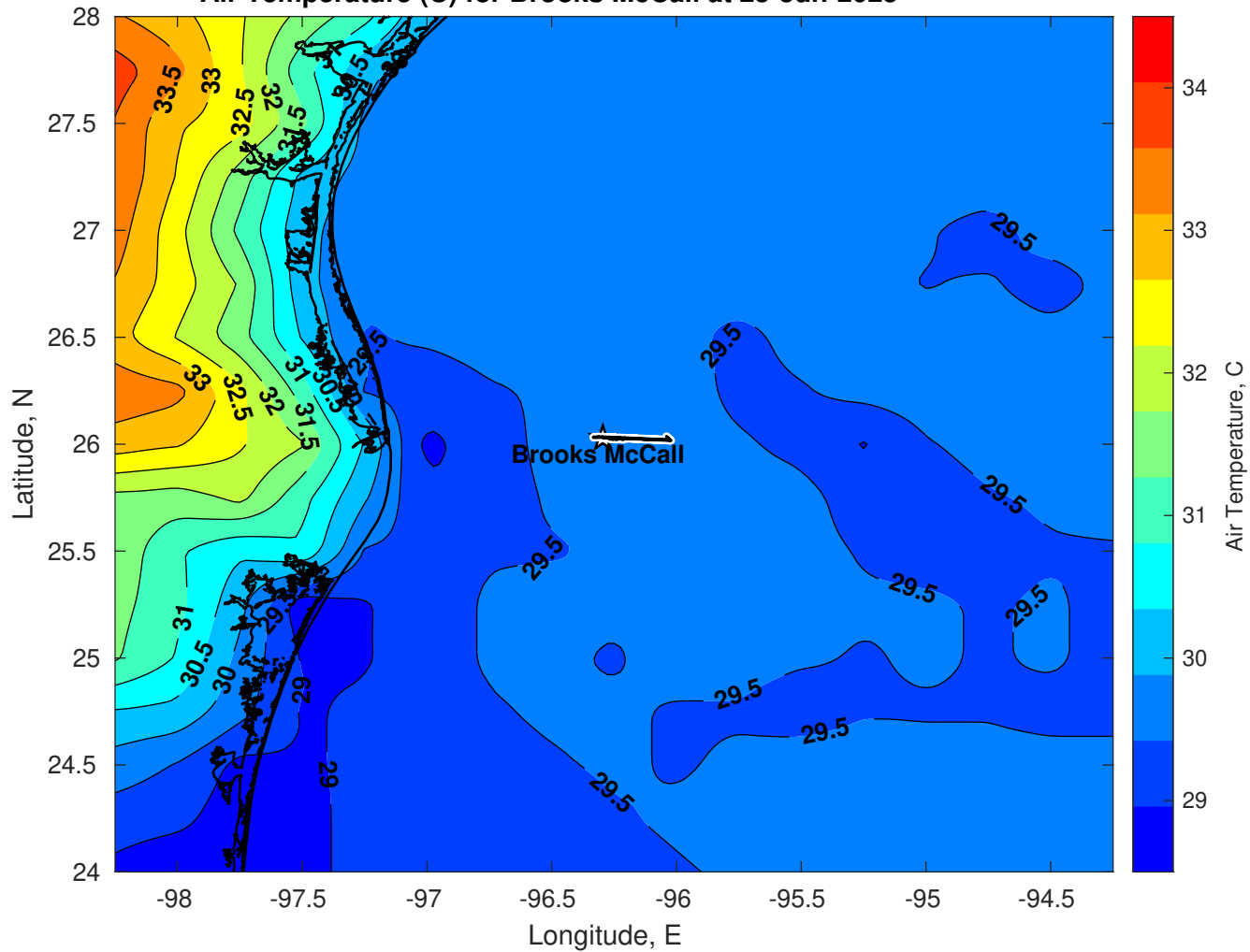
Air Temperature (C) for Brooks McCall at 25-Jun-2025
