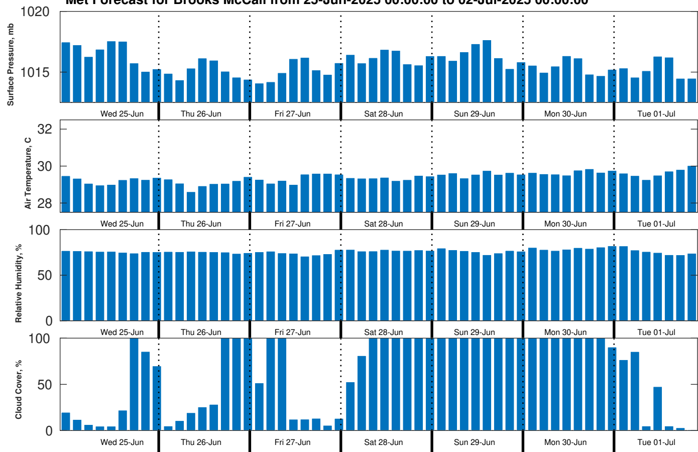
Met Forecast for Brooks McCall from 25-Jun-2025 00:00:00 to 02-Jul-2025 00:00:00
