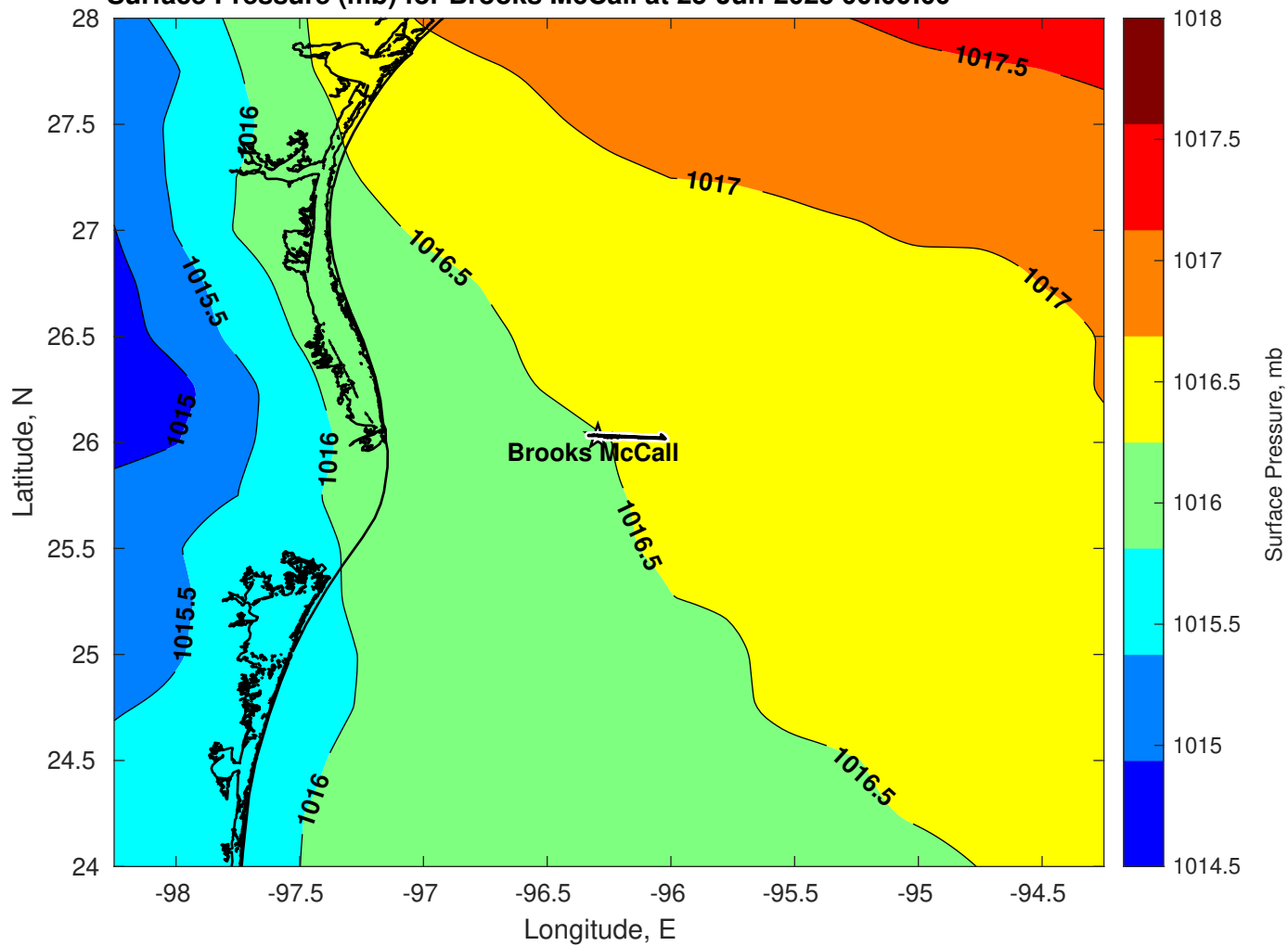
Surface Pressure (mb) for Brooks McCall at 25-Jun-2025 00:00:00
