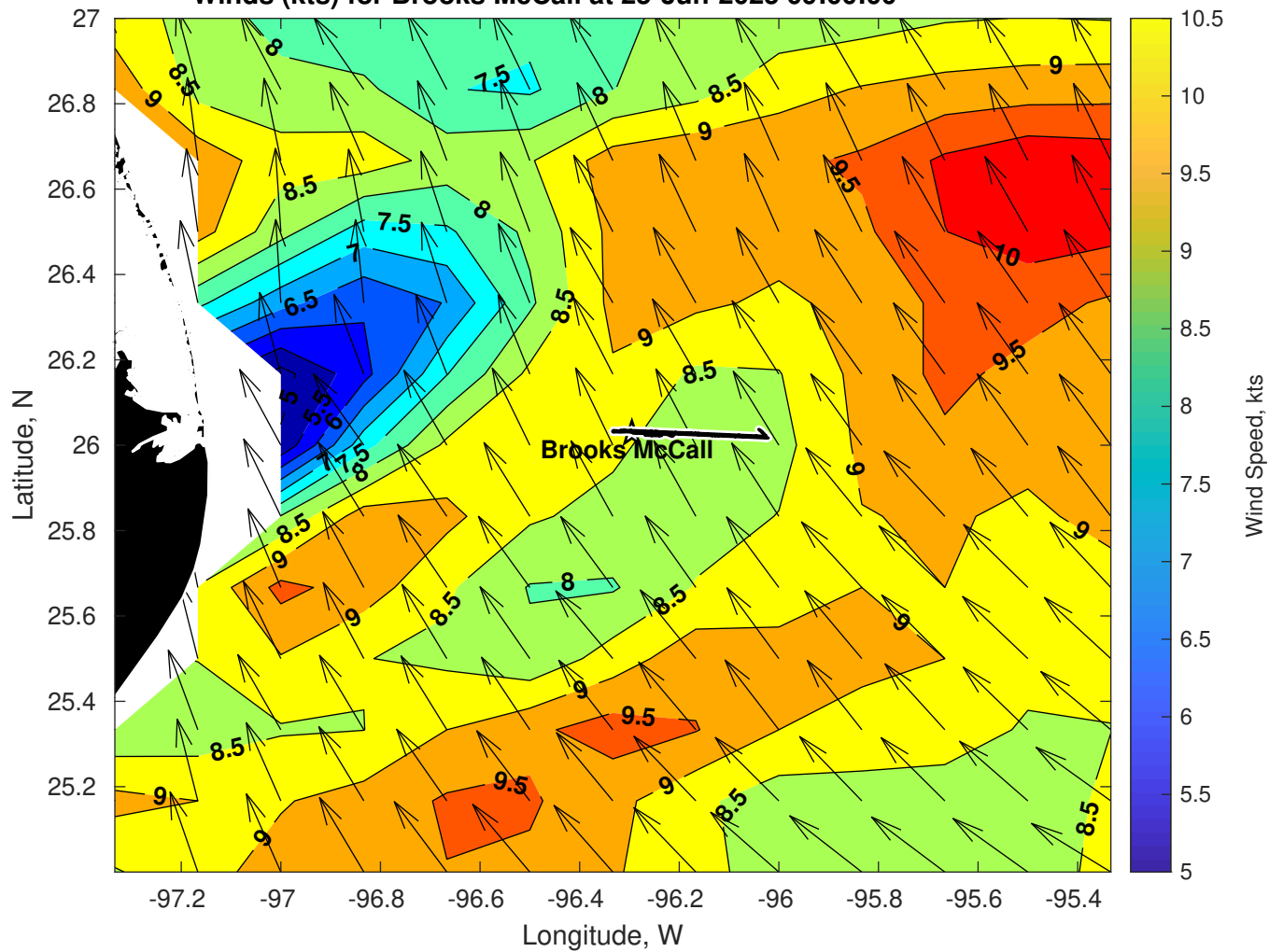
Winds (kts) for Brooks McCall at 25-Jun-2025 09:00:00
