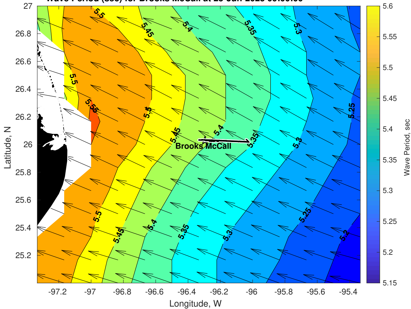
Wave Period (sec) for Brooks McCall at 25-Jun-2025 09:00:00
