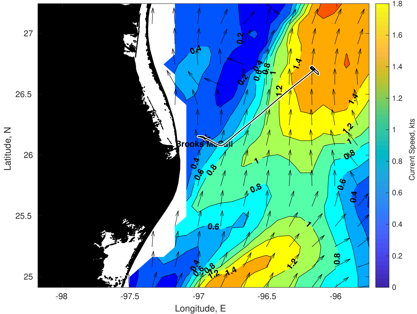
Surface Currents for Brooks McCall at 23-Jun-2025 00:00:00
