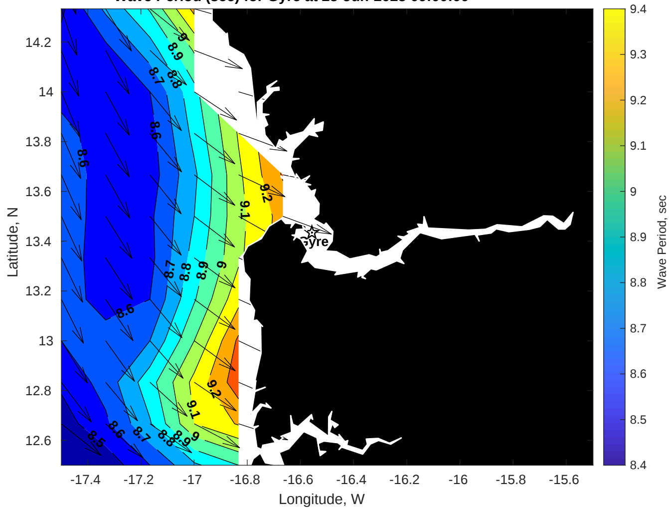
Wave Period (sec) for Gyre at 25-Jun-2025 09:00:00
