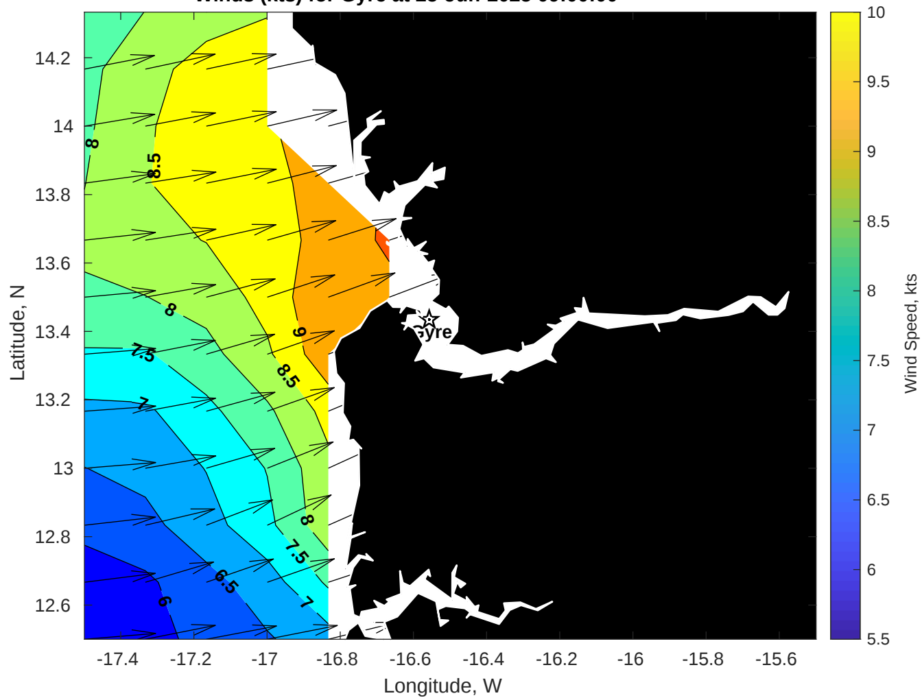
Winds (kts) for Gyre at 25-Jun-2025 09:00:00
