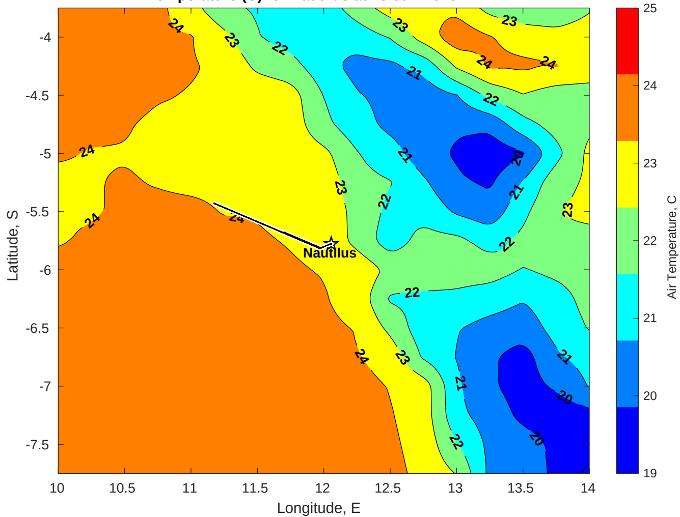
Air Temperature (C) for Nautilus at 25-Jun-2025
