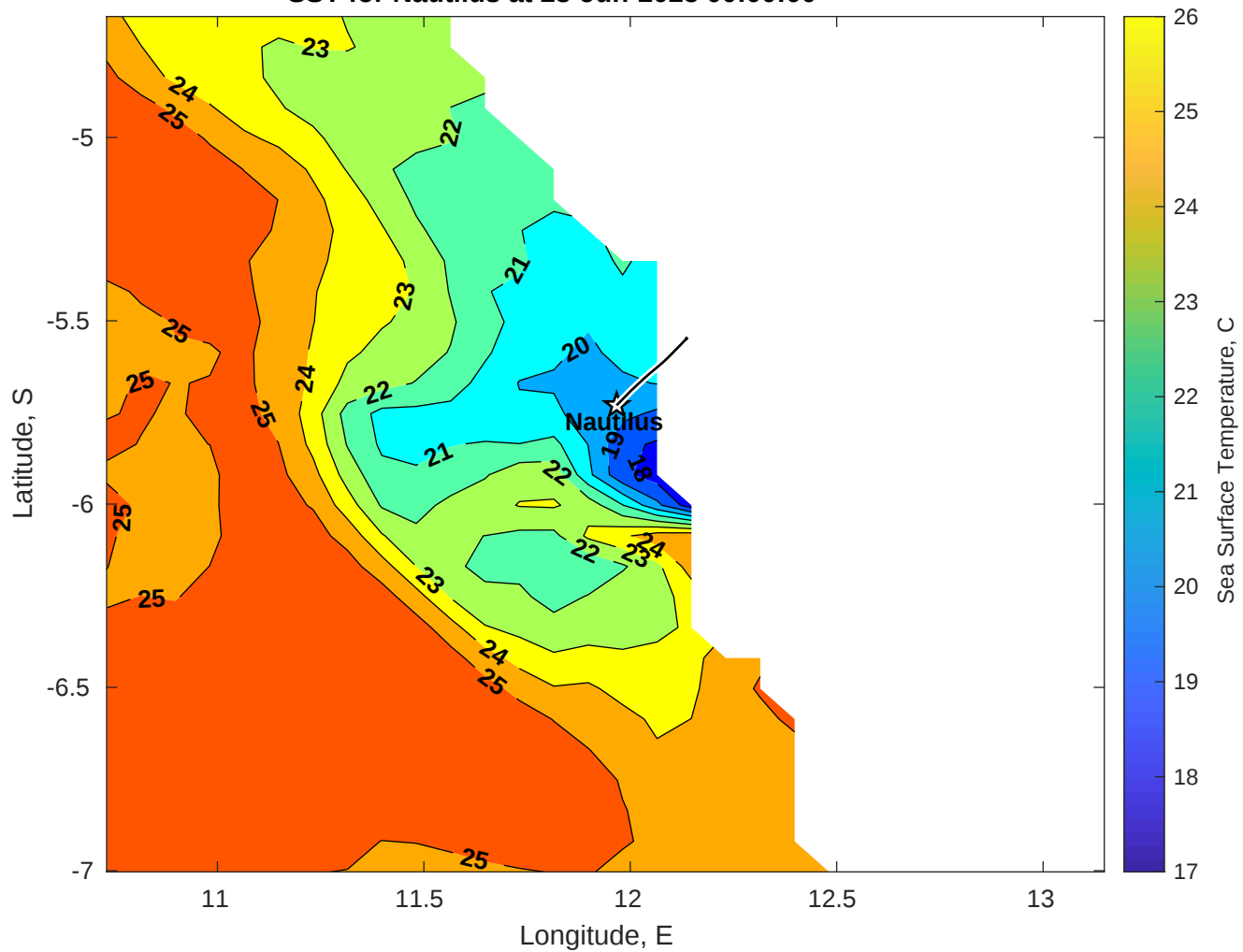
SST for Nautilus at 23-Jun-2025 00:00:00
