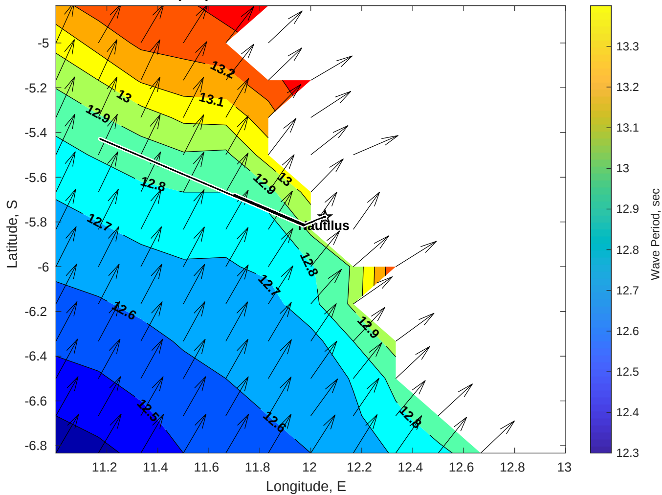
Wave Period (sec) for Nautilus at 25-Jun-2025 09:00:00
