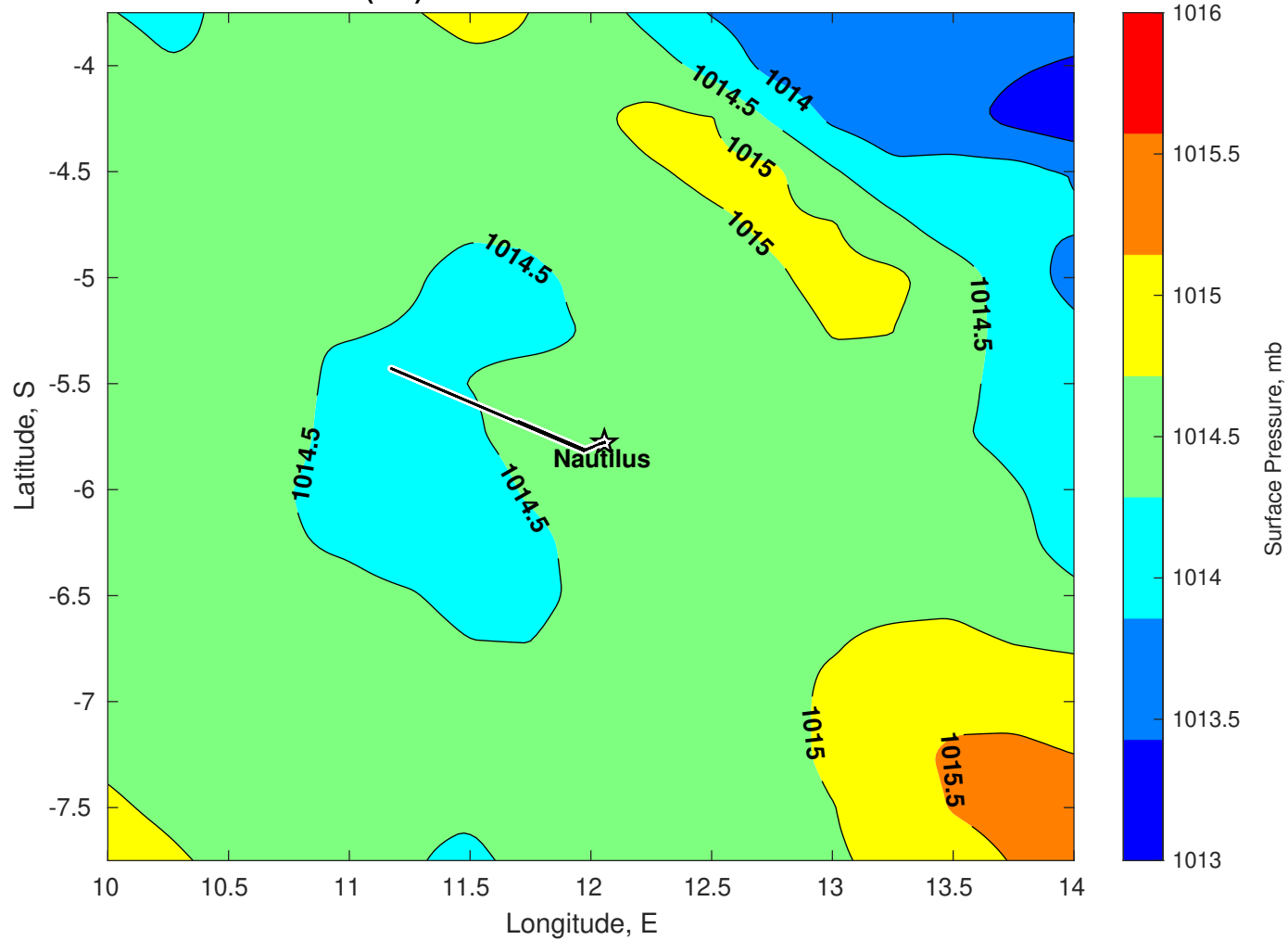
Surface Pressure (mb) for Nautilus at 26-Jun-2025 00:00:00
