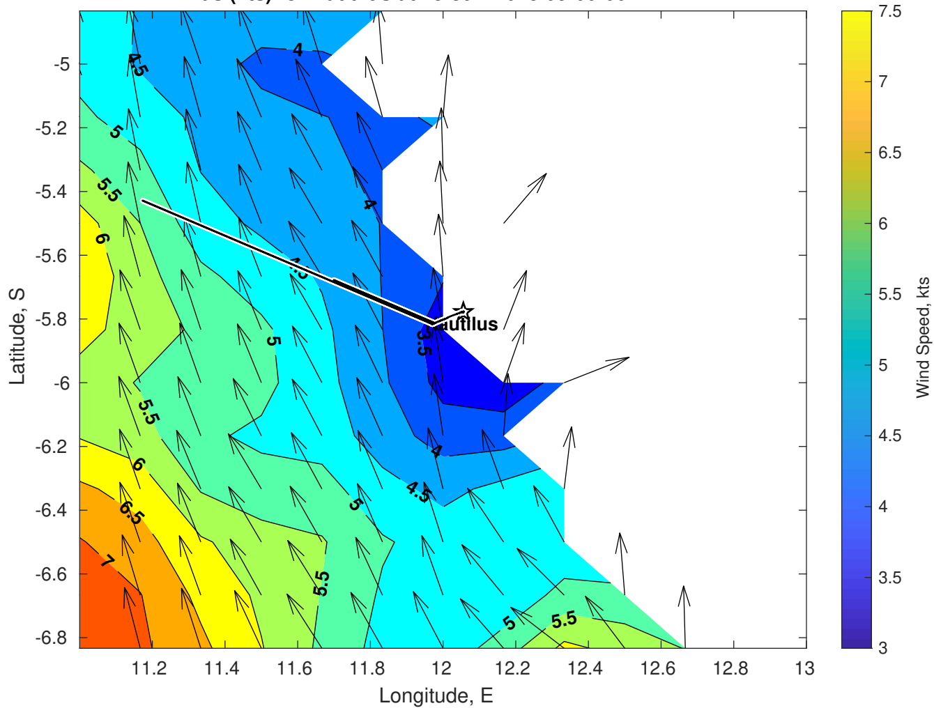
Winds (kts) for Nautilus at 25-Jun-2025 09:00:00
