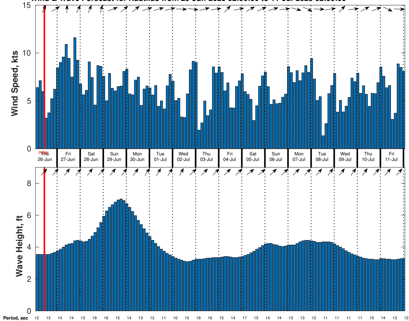
Wind & Wave Forecast for Nautilus from 25-Jun-2025 02:00:00 to 11-Jul-2025 02:00:00
