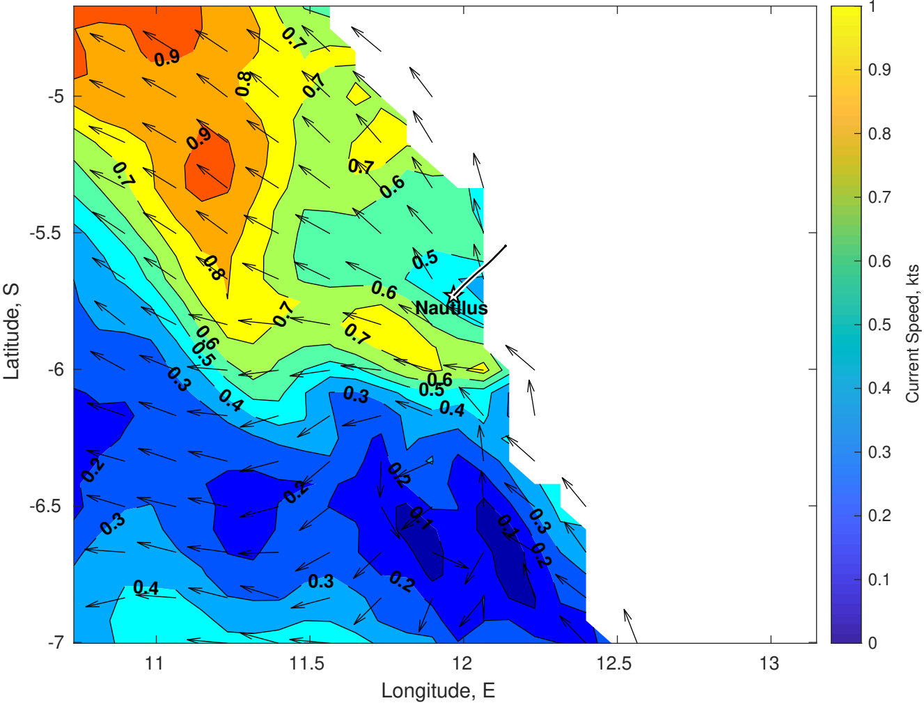
Surface Currents for Nautilus at 23-Jun-2025 00:00:00
