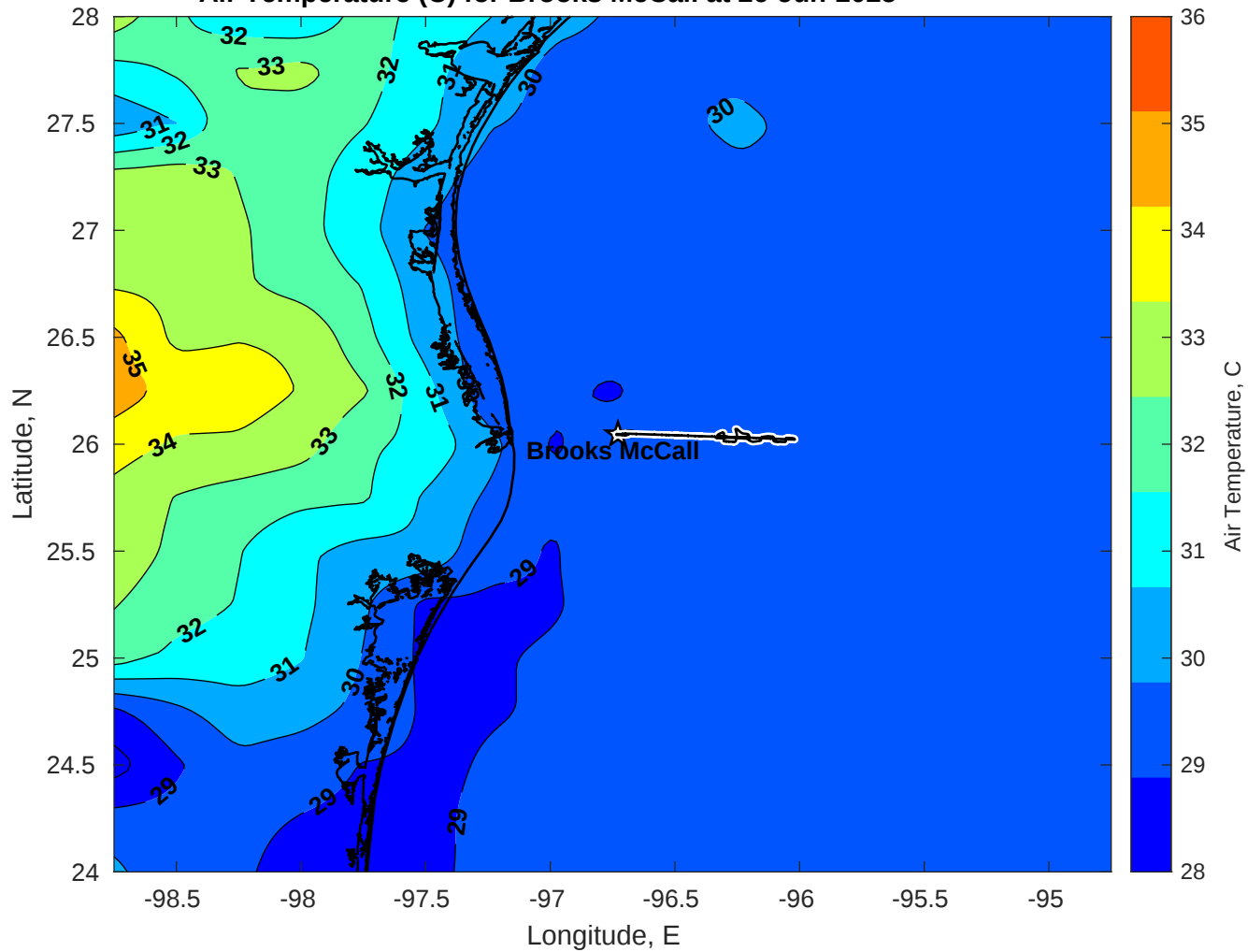
Air Temperature (C) for Brooks McCall at 26-Jun-2025
