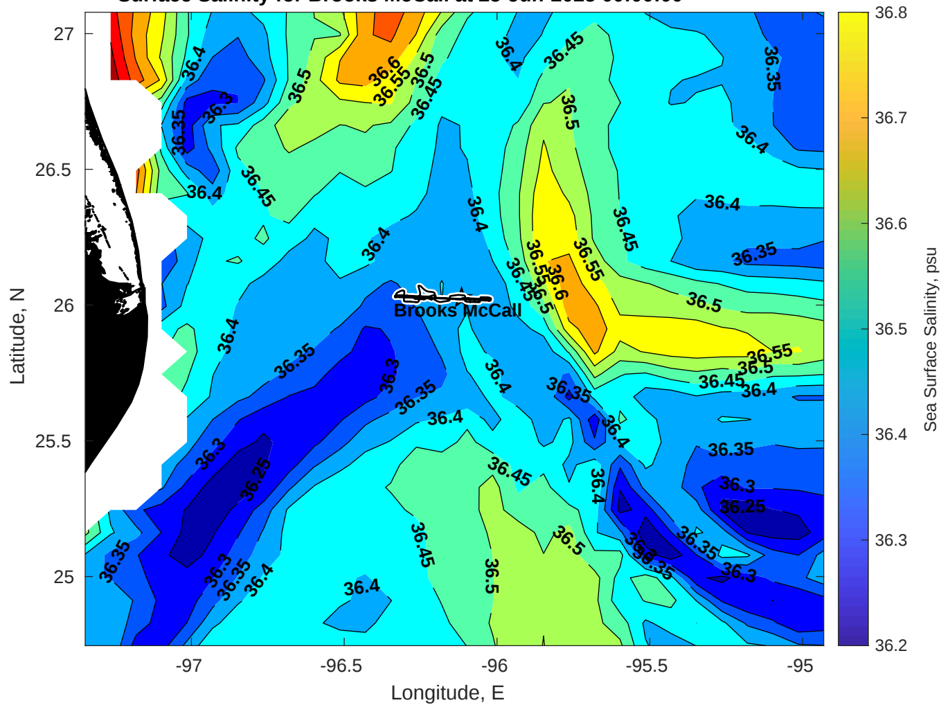
Surface Salinity for Brooks McCall at 25-Jun-2025 00:00:00
