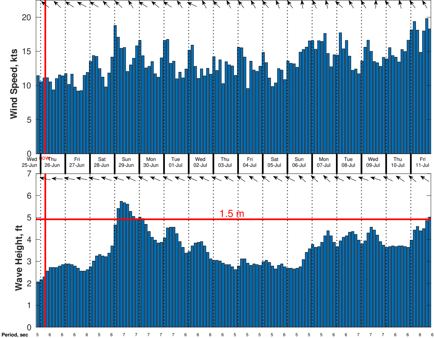
Wind & Wave Forecast for Brooks McCall from 25-Jun-2025 20:00:00 to 11-Jul-2025 20:00:00
