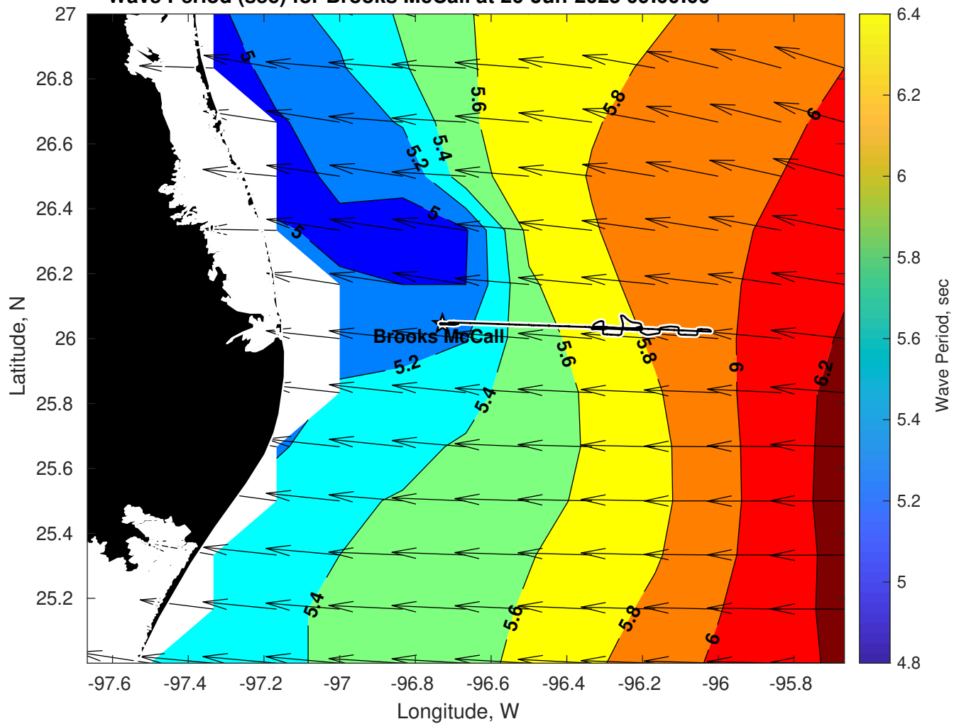
Wave Period (sec) for Brooks McCall at 26-Jun-2025 09:00:00
