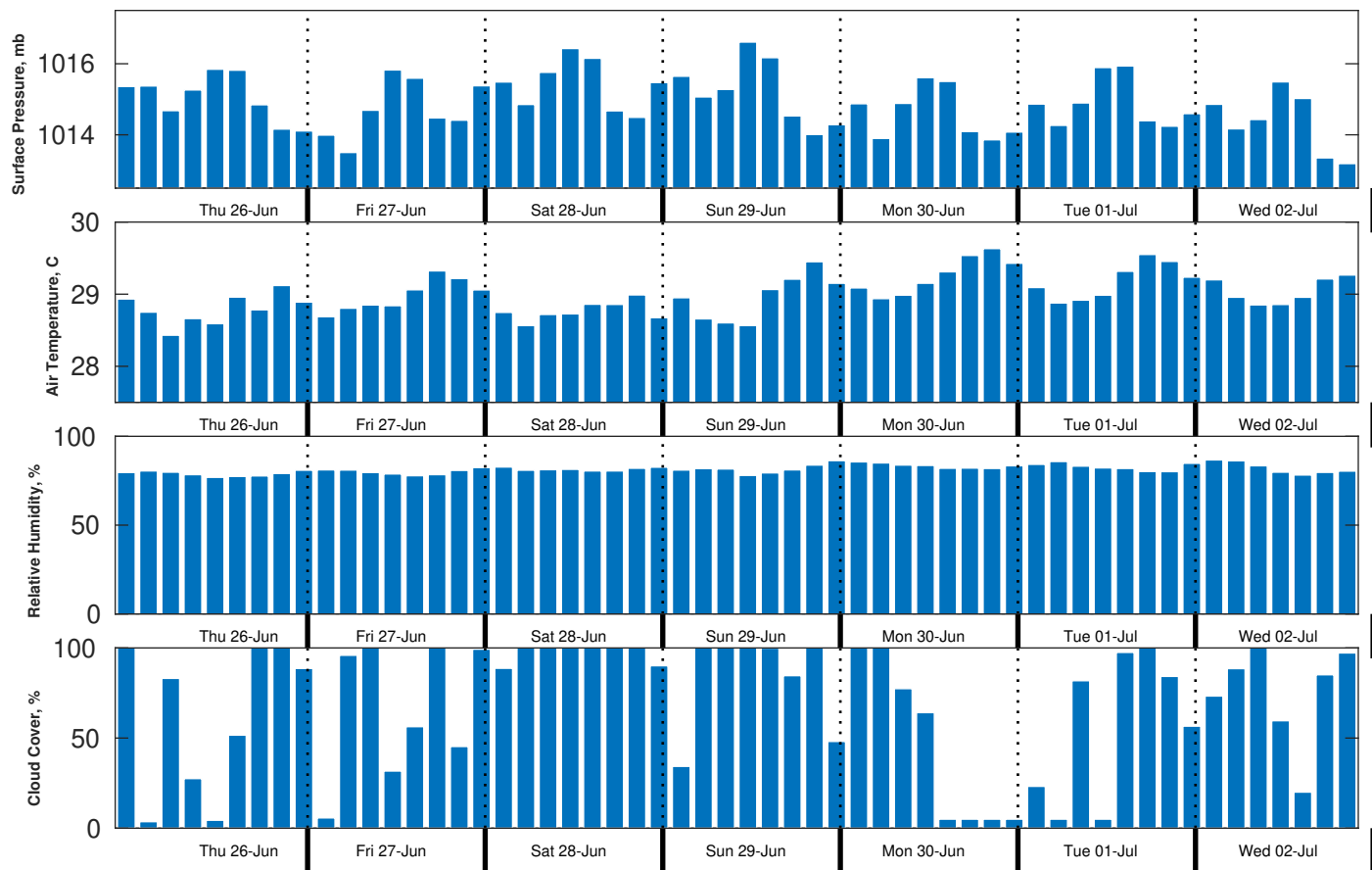
Met Forecast for Brooks McCall from 26-Jun-2025 00:00:00 to 03-Jul-2025 00:00:00
