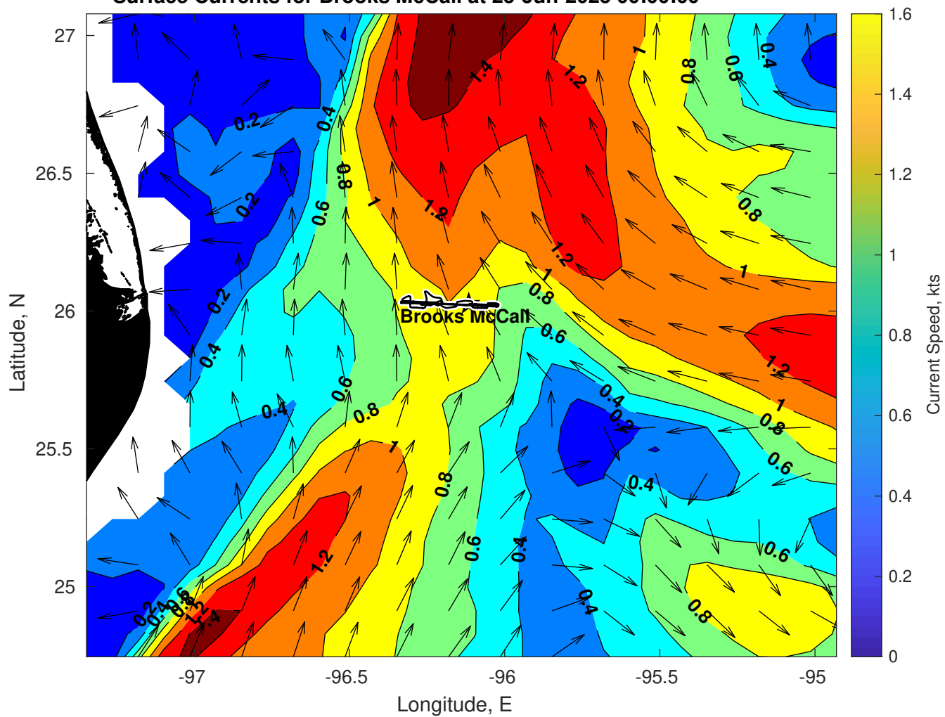
Surface Currents for Brooks McCall at 25-Jun-2025 00:00:00
