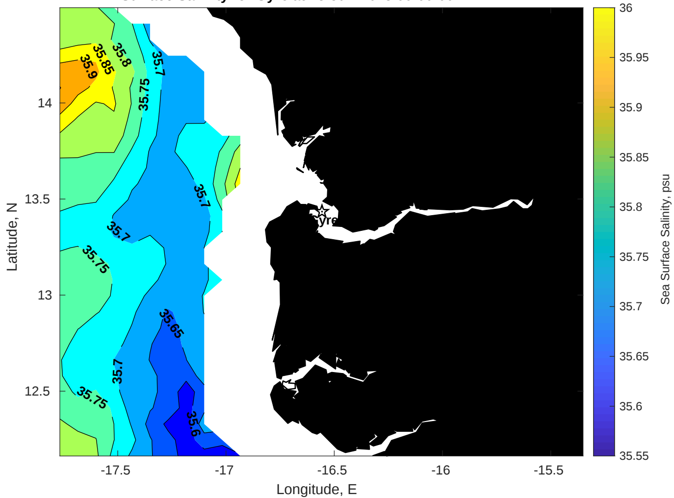
Surface Salinity for Gyre at 25-Jun-2025 00:00:00
