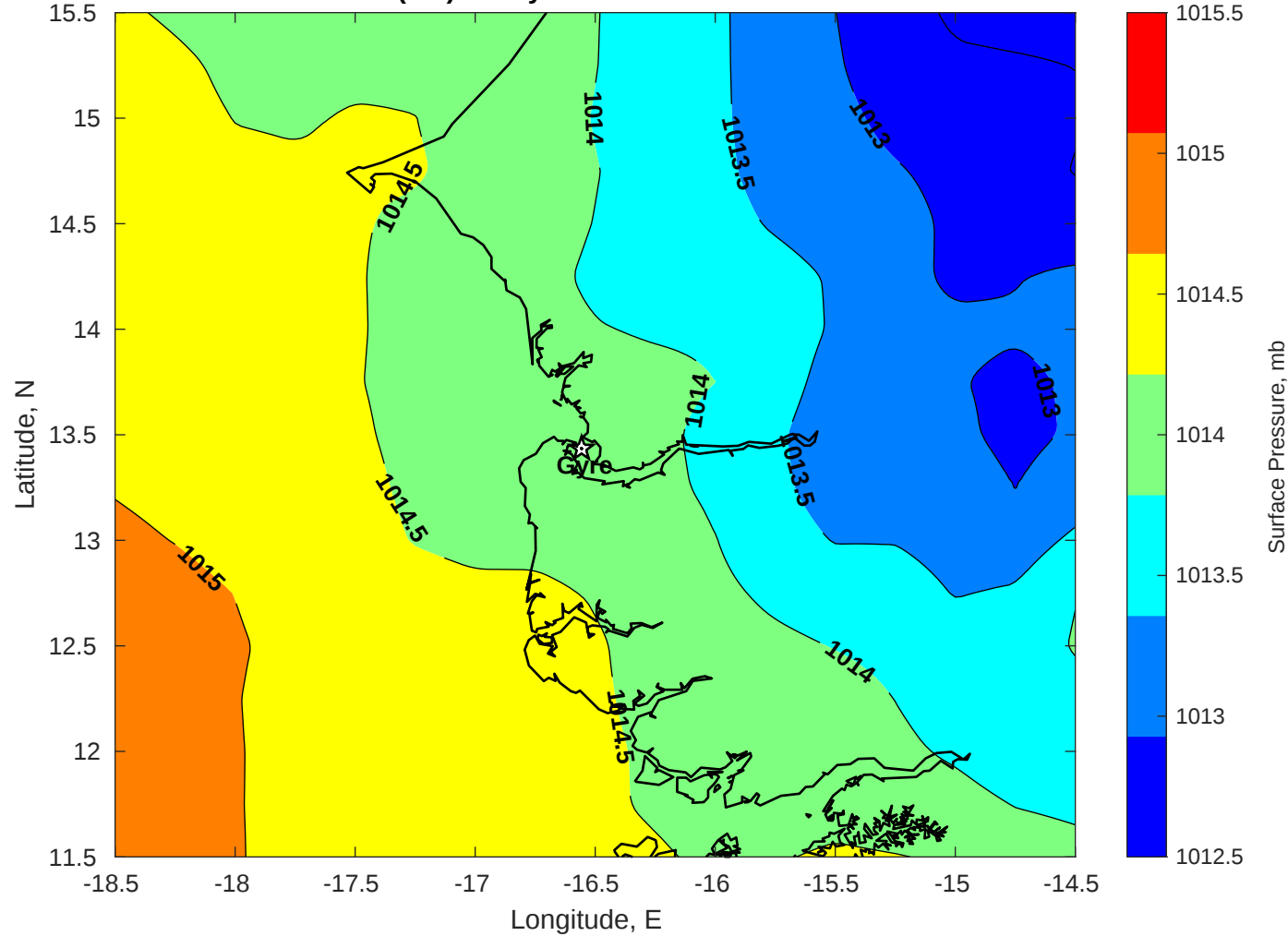
Surface Pressure (mb) for Gyre at 26-Jun-2025 00:00:00
