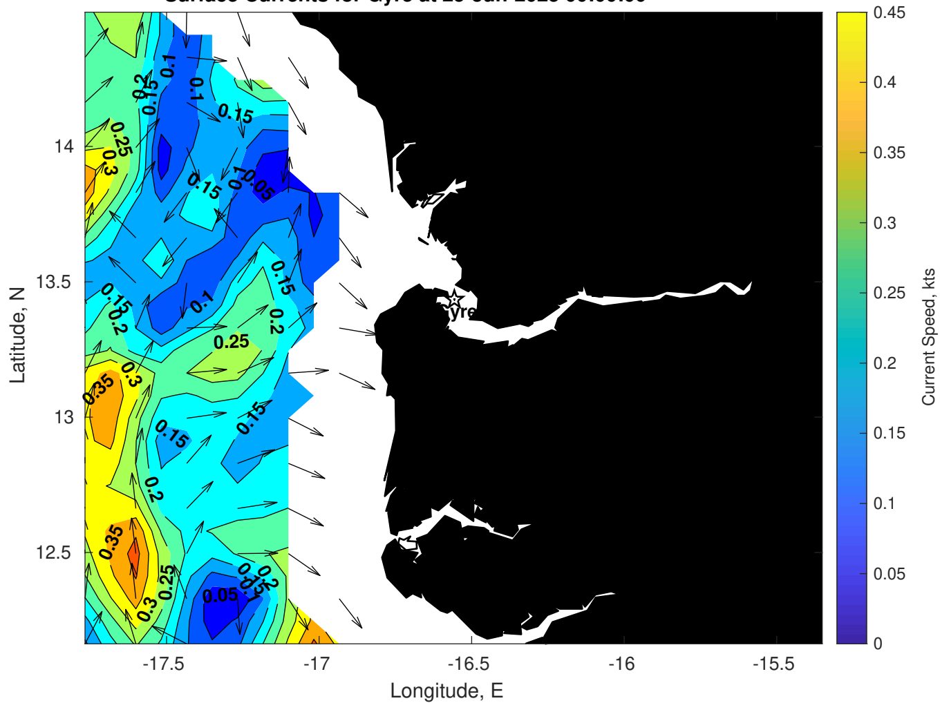
Surface Currents for Gyre at 25-Jun-2025 00:00:00
