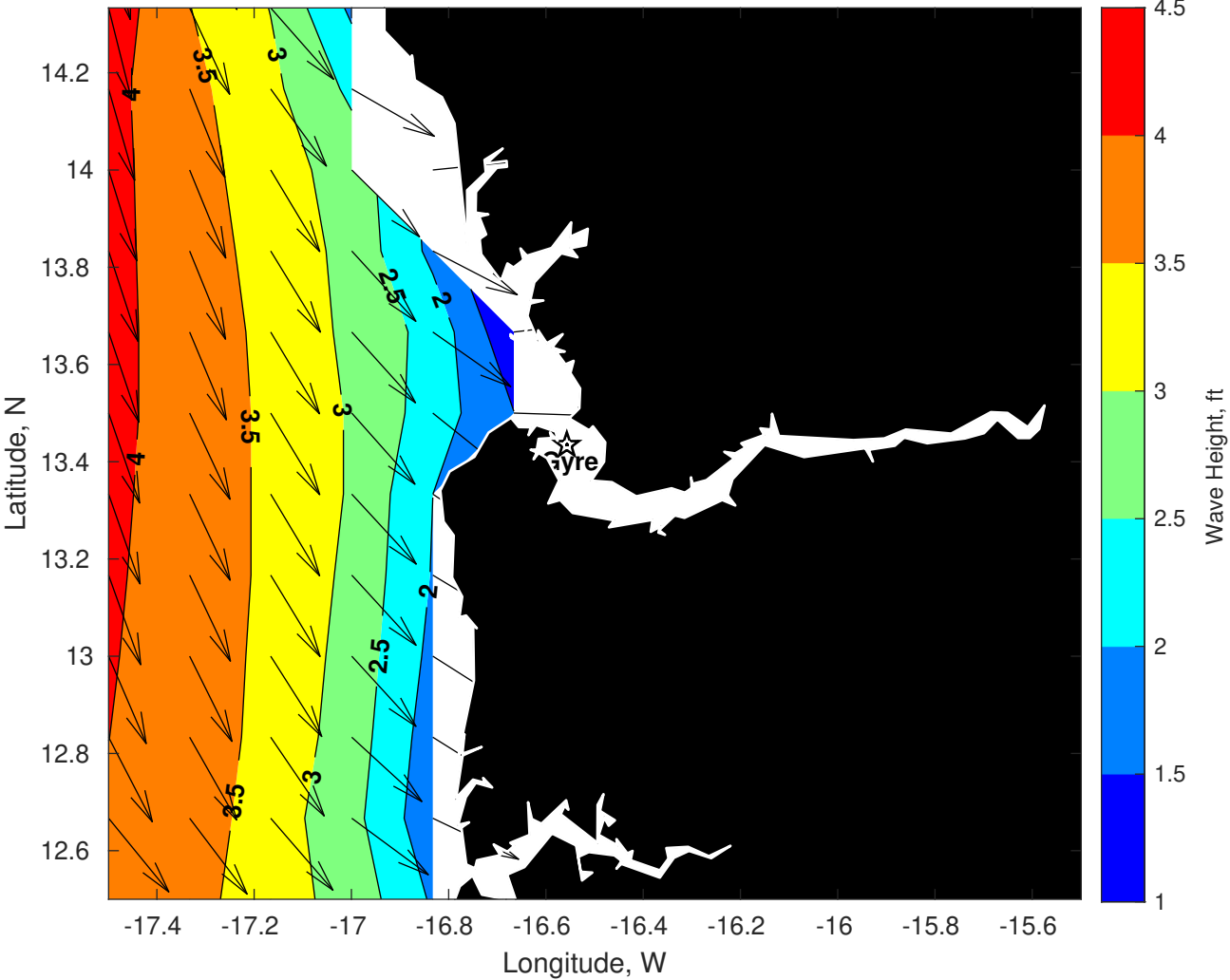
Wave Height (ft) for Gyre at 26-Jun-2025 09:00:00
