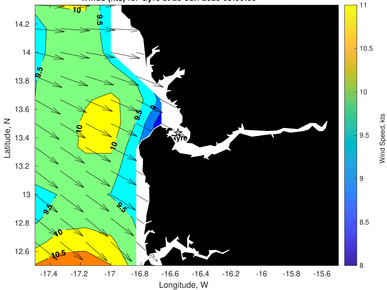
Winds (kts) for Gyre at 26-Jun-2025 09:00:00
