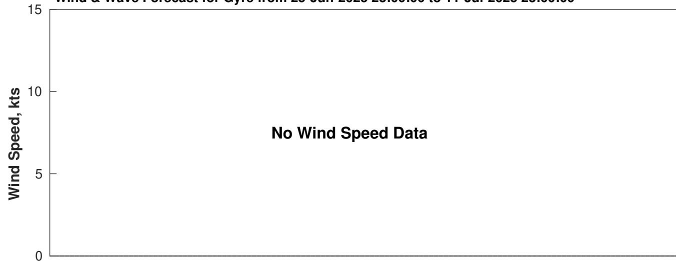
Wind & Wave Forecast for Gyre from 25-Jun-2025 23:00:00 to 11-Jul-2025 23:00:00
