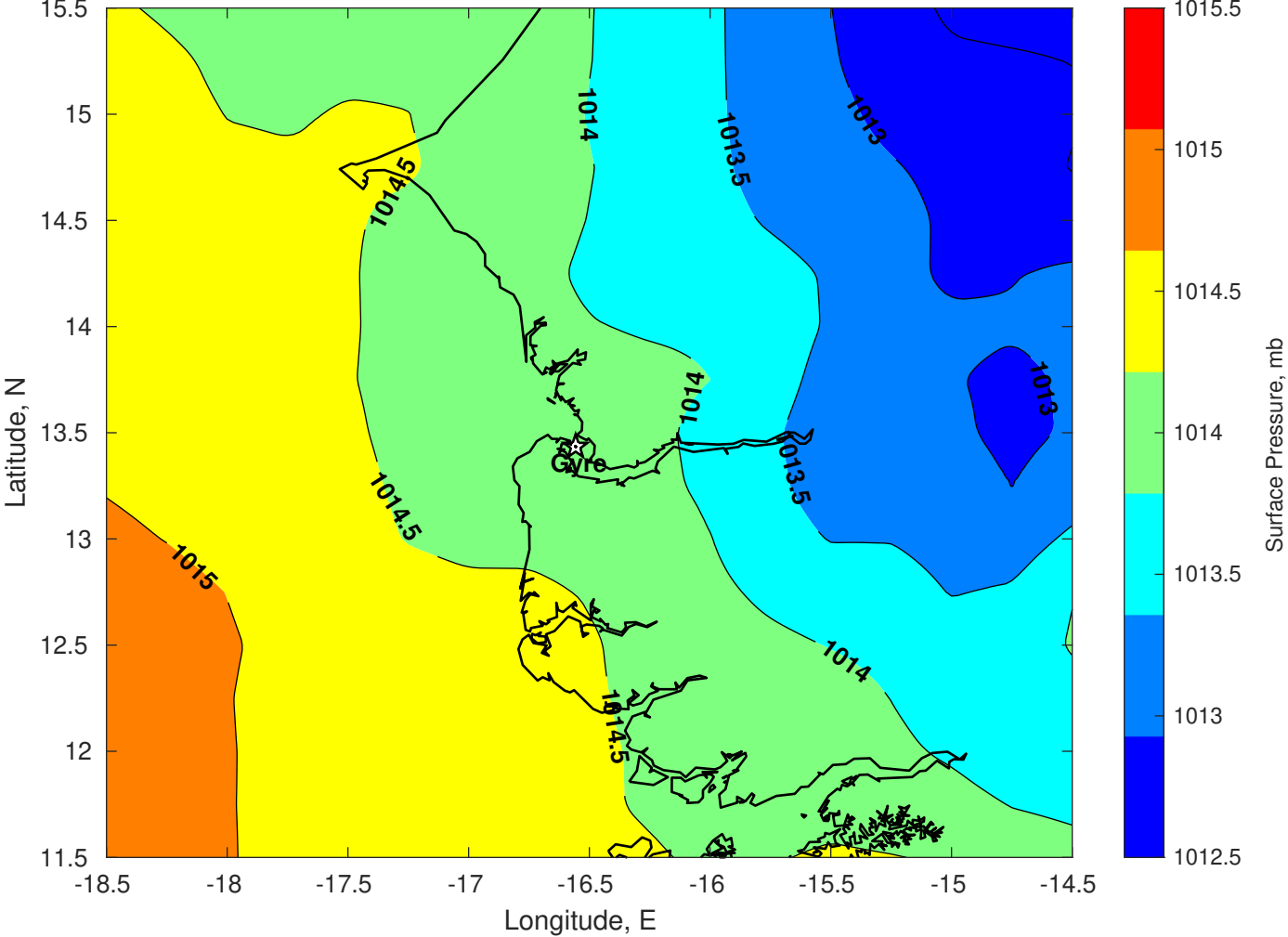
Surface Pressure (mb) for Gyre at 26-Jun-2025 00:00:00
