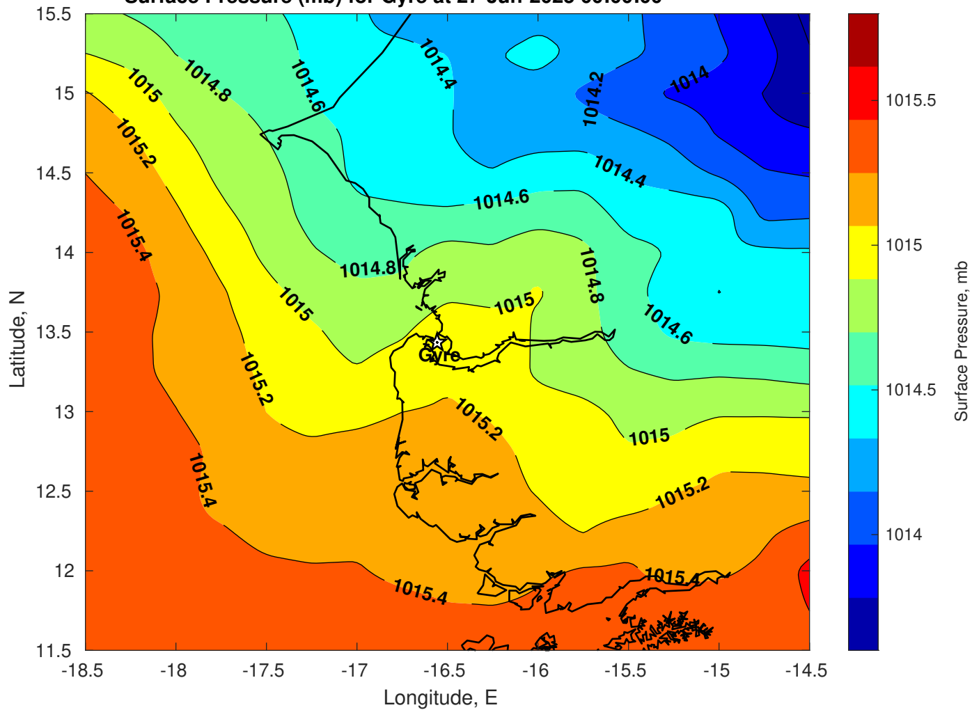
Surface Pressure (mb) for Gyre at 27-Jun-2025 00:00:00
