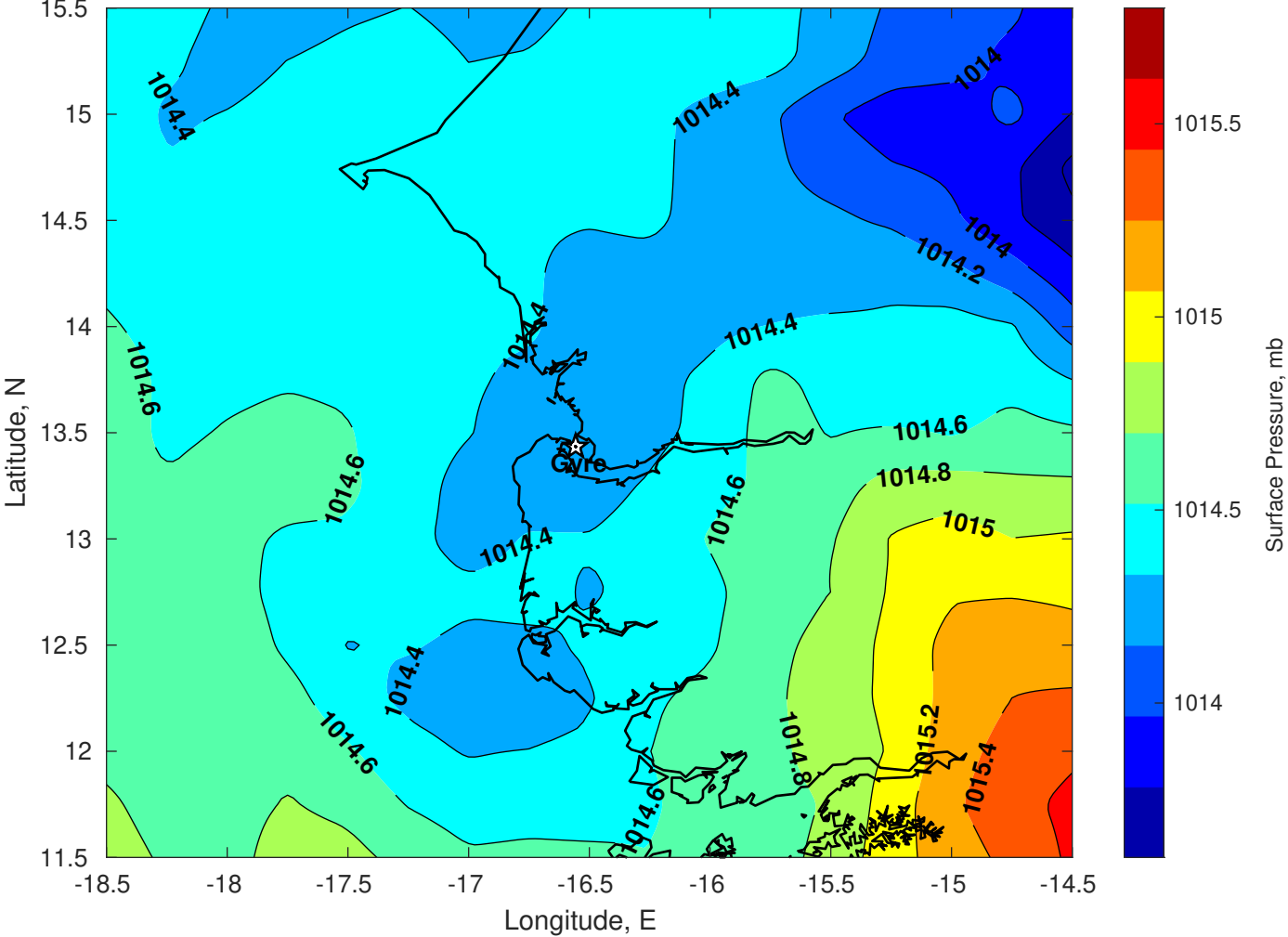
Surface Pressure (mb) for Gyre at 28-Jun-2025 00:00:00
