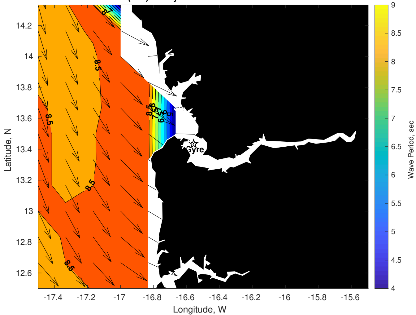
Wave Period (sec) for Gyre at 26-Jun-2025 09:00:00
