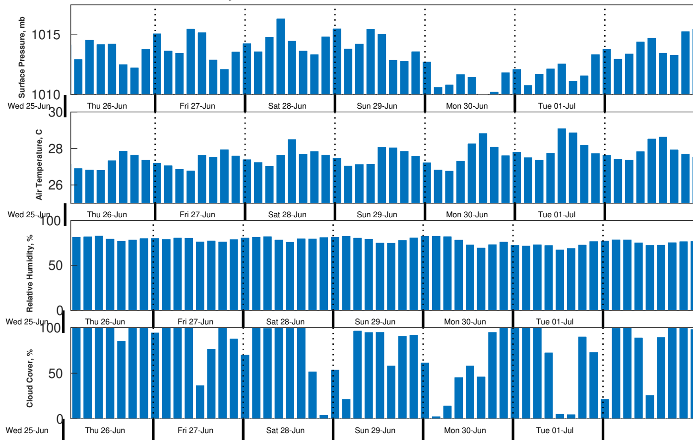
Met Forecast for Gyre from 25-Jun-2025 23:00:00 to 02-Jul-2025 23:00:00
