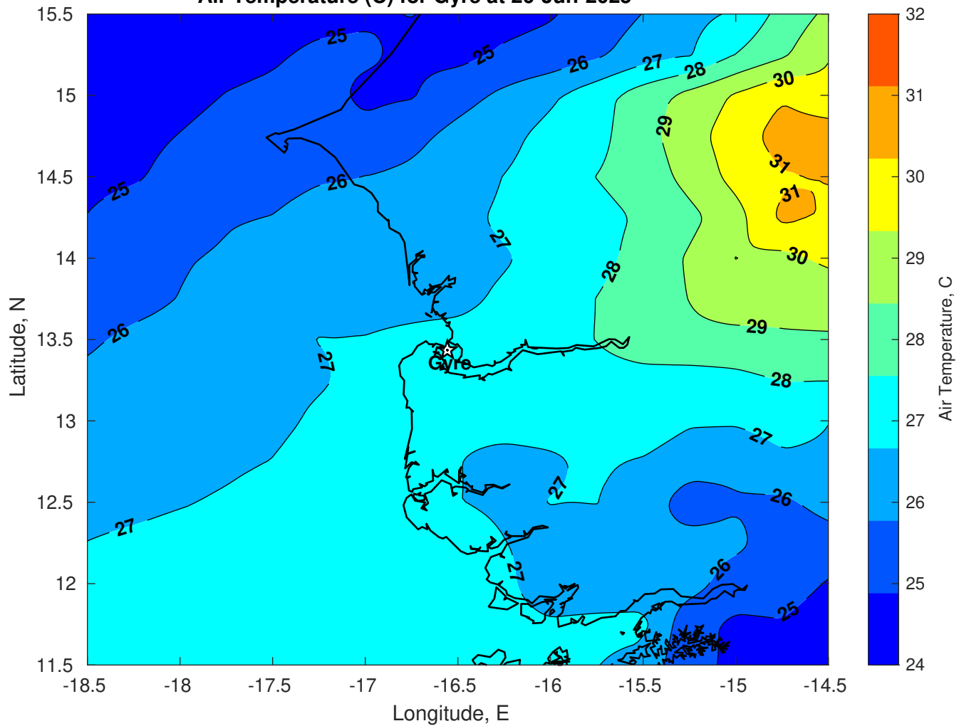
Air Temperature (C) for Gyre at 26-Jun-2025
