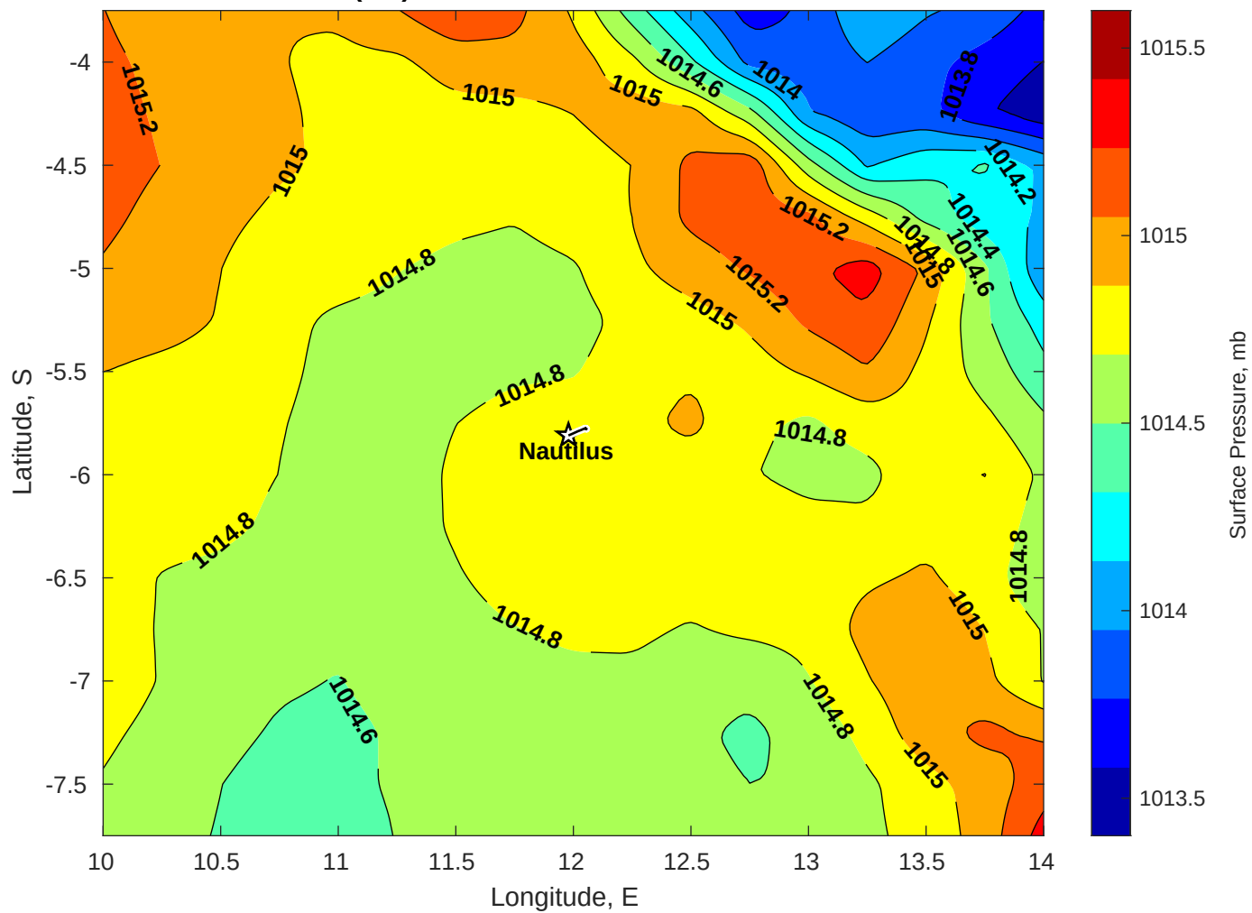
Surface Pressure (mb) for Nautilus at 28-Jun-2025 00:00:00
