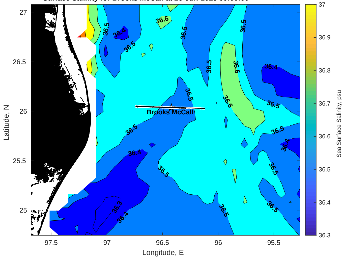
Surface Salinity for Brooks McCall at 26-Jun-2025 00:00:00
