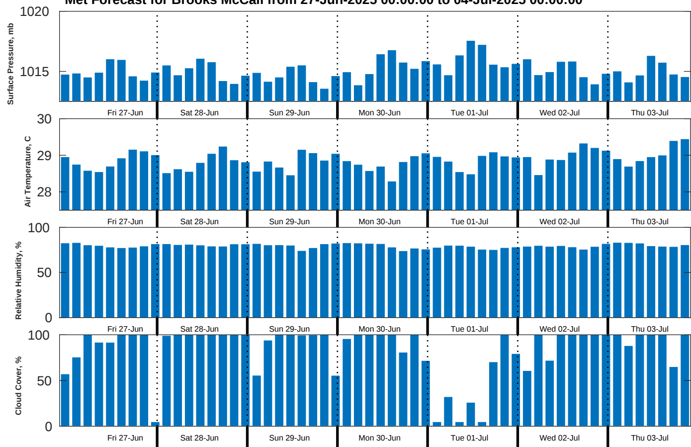
Met Forecast for Brooks McCall from 27-Jun-2025 00:00:00 to 04-Jul-2025 00:00:00
