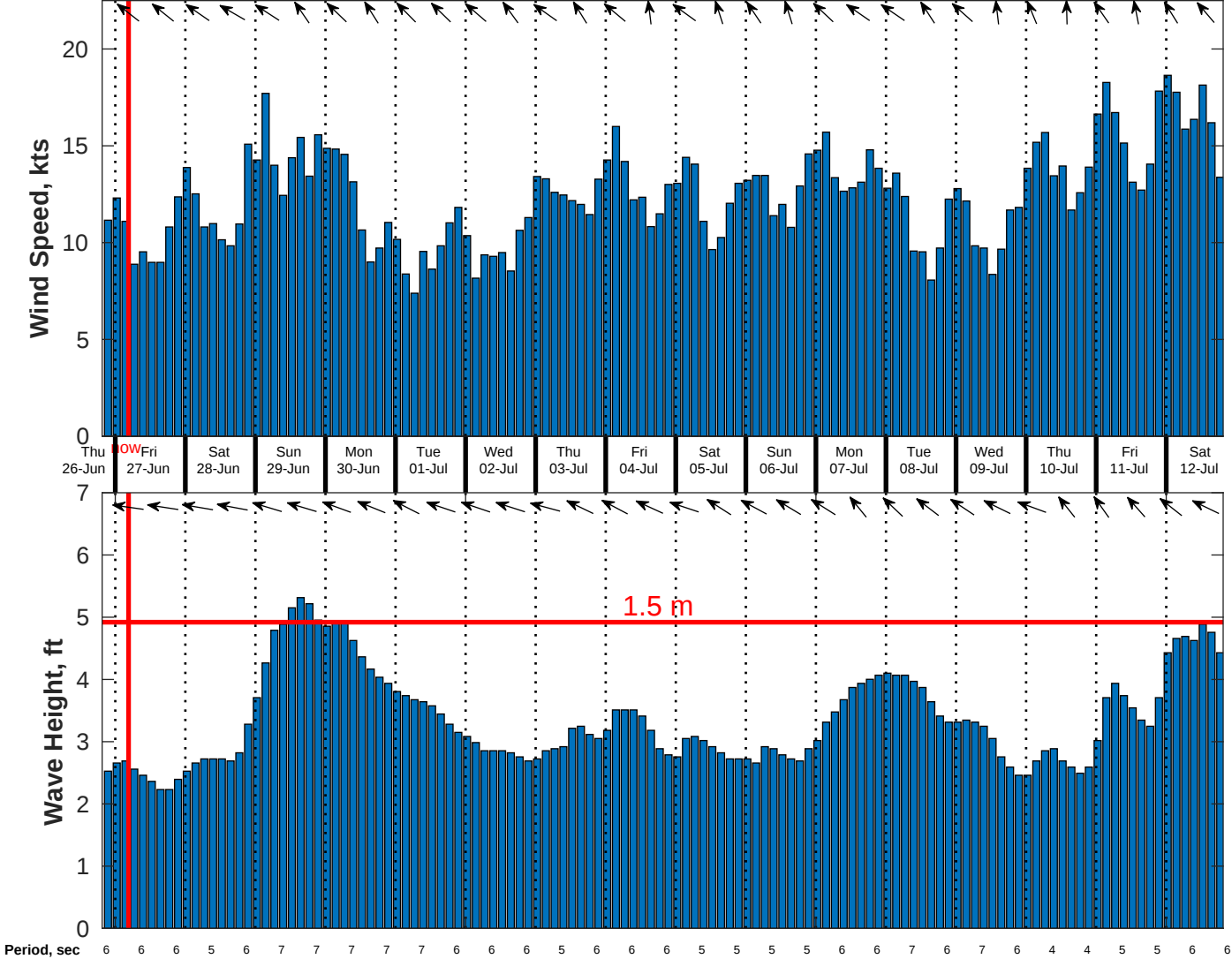
Wind & Wave Forecast for Brooks McCall from 26-Jun-2025 20:00:00 to 12-Jul-2025 20:00:00
