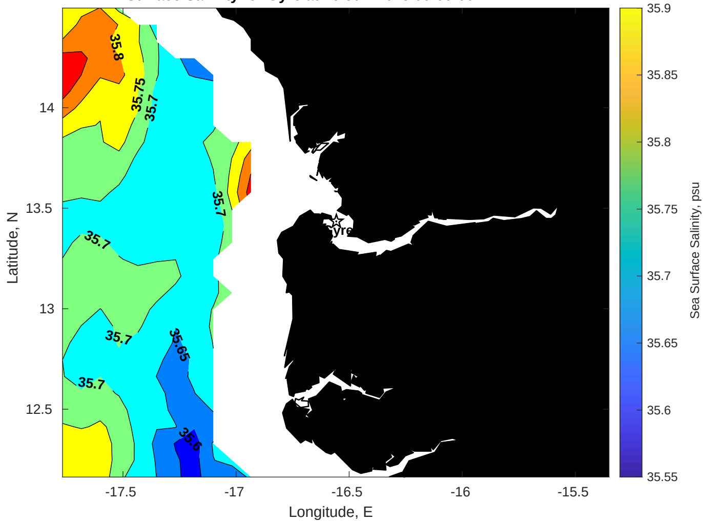
Surface Salinity for Gyre at 26-Jun-2025 00:00:00
