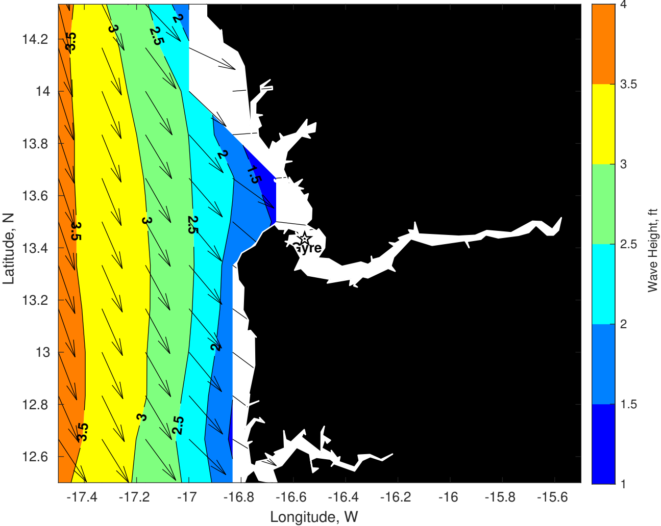
Wave Height (ft) for Gyre at 27-Jun-2025 09:00:00
