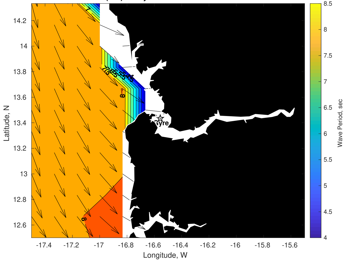
Wave Period (sec) for Gyre at 27-Jun-2025 09:00:00
