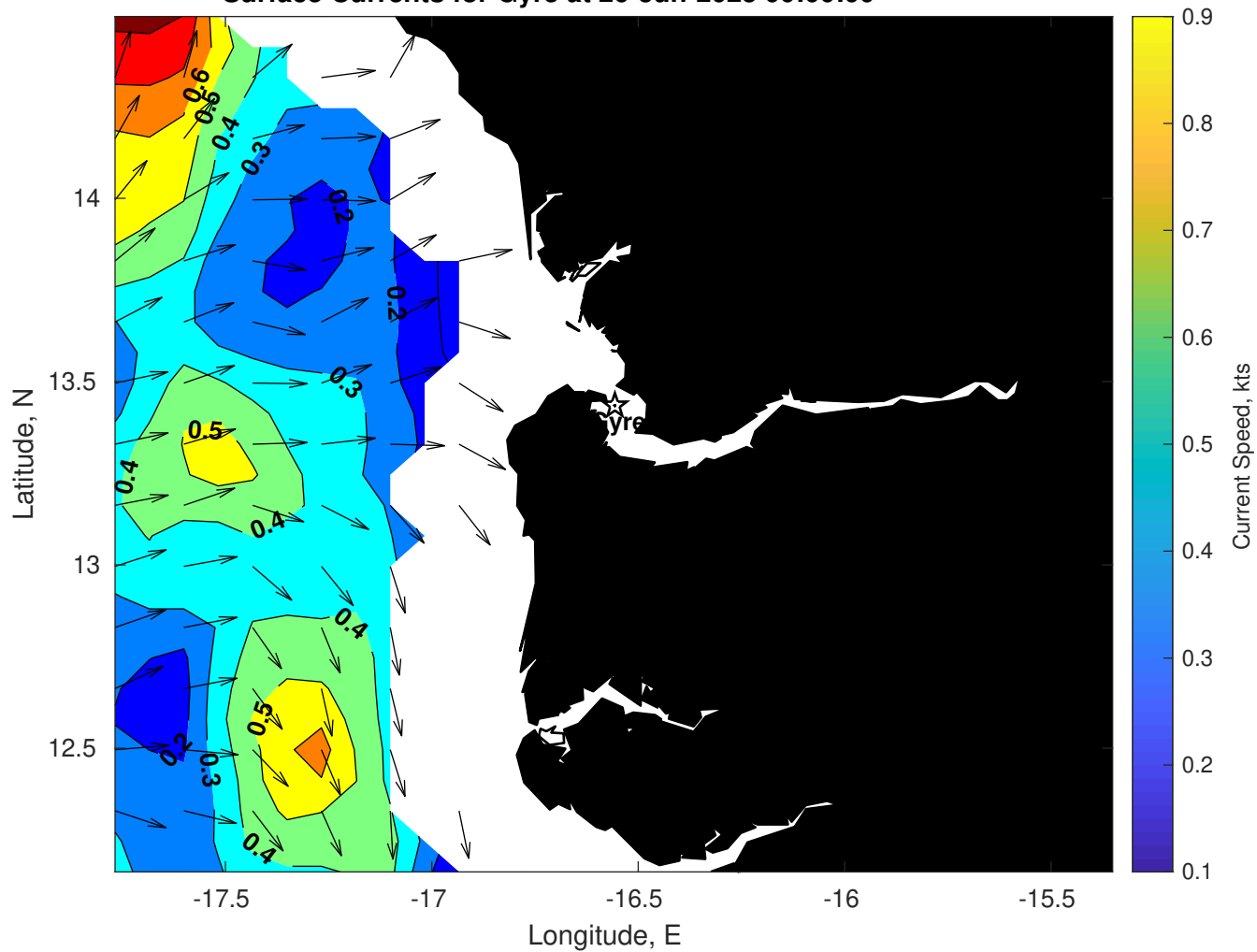
Surface Currents for Gyre at 26-Jun-2025 00:00:00
