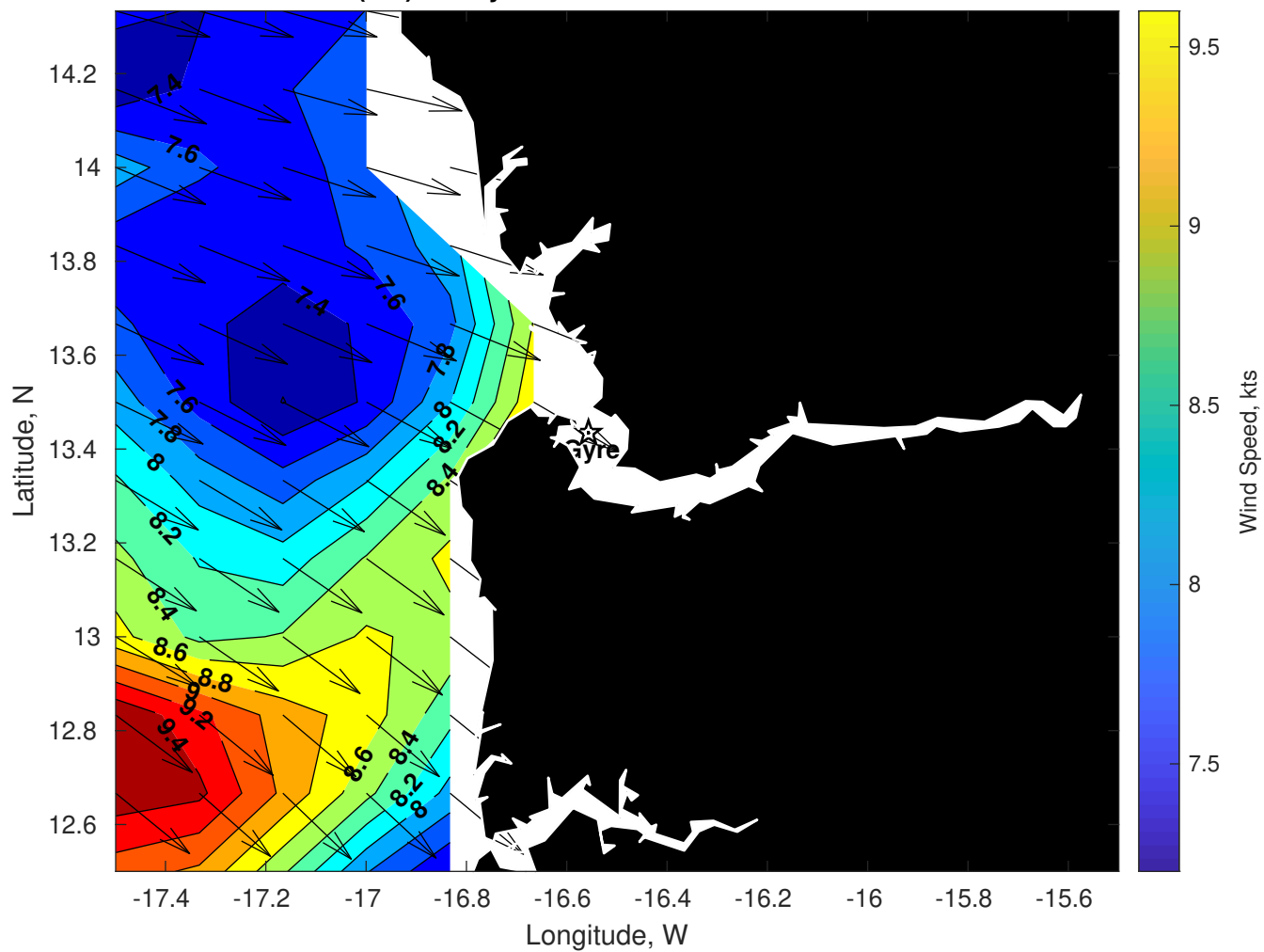
Winds (kts) for Gyre at 27-Jun-2025 09:00:00
