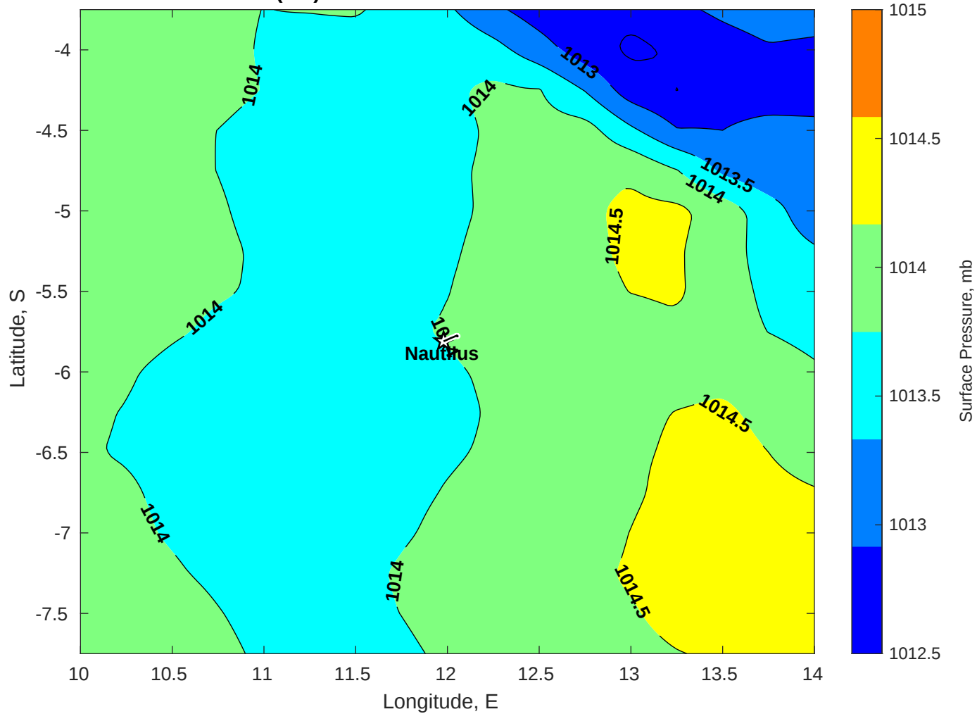
Surface Pressure (mb) for Nautilus at 27-Jun-2025 00:00:00
