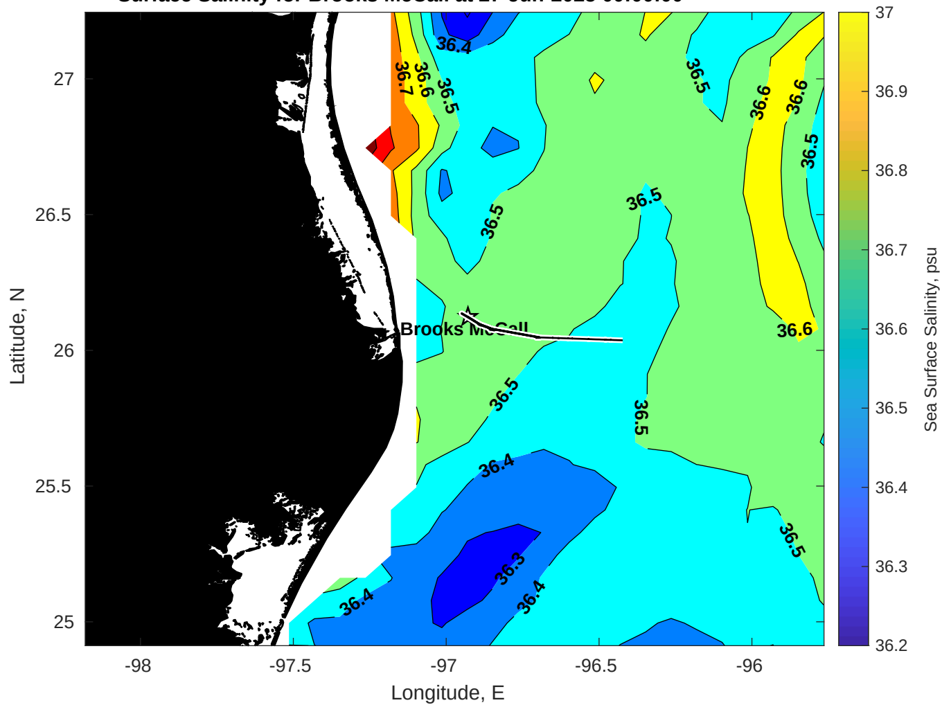
Surface Salinity for Brooks McCall at 27-Jun-2025 00:00:00
