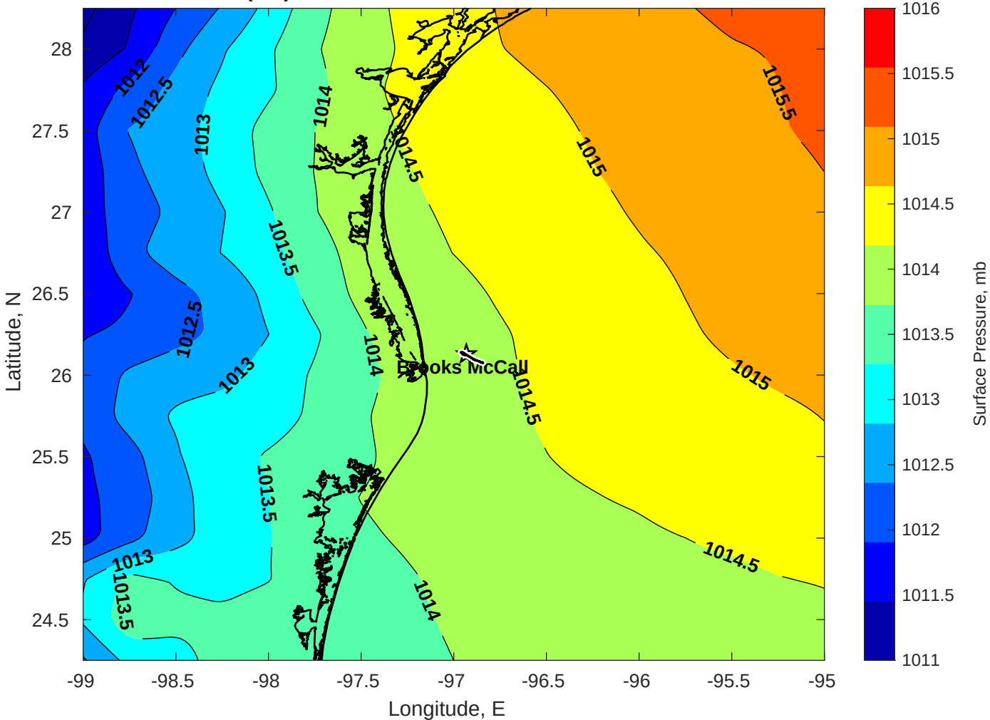
Surface Pressure (mb) for Brooks McCall at 28-Jun-2025 00:00:00
