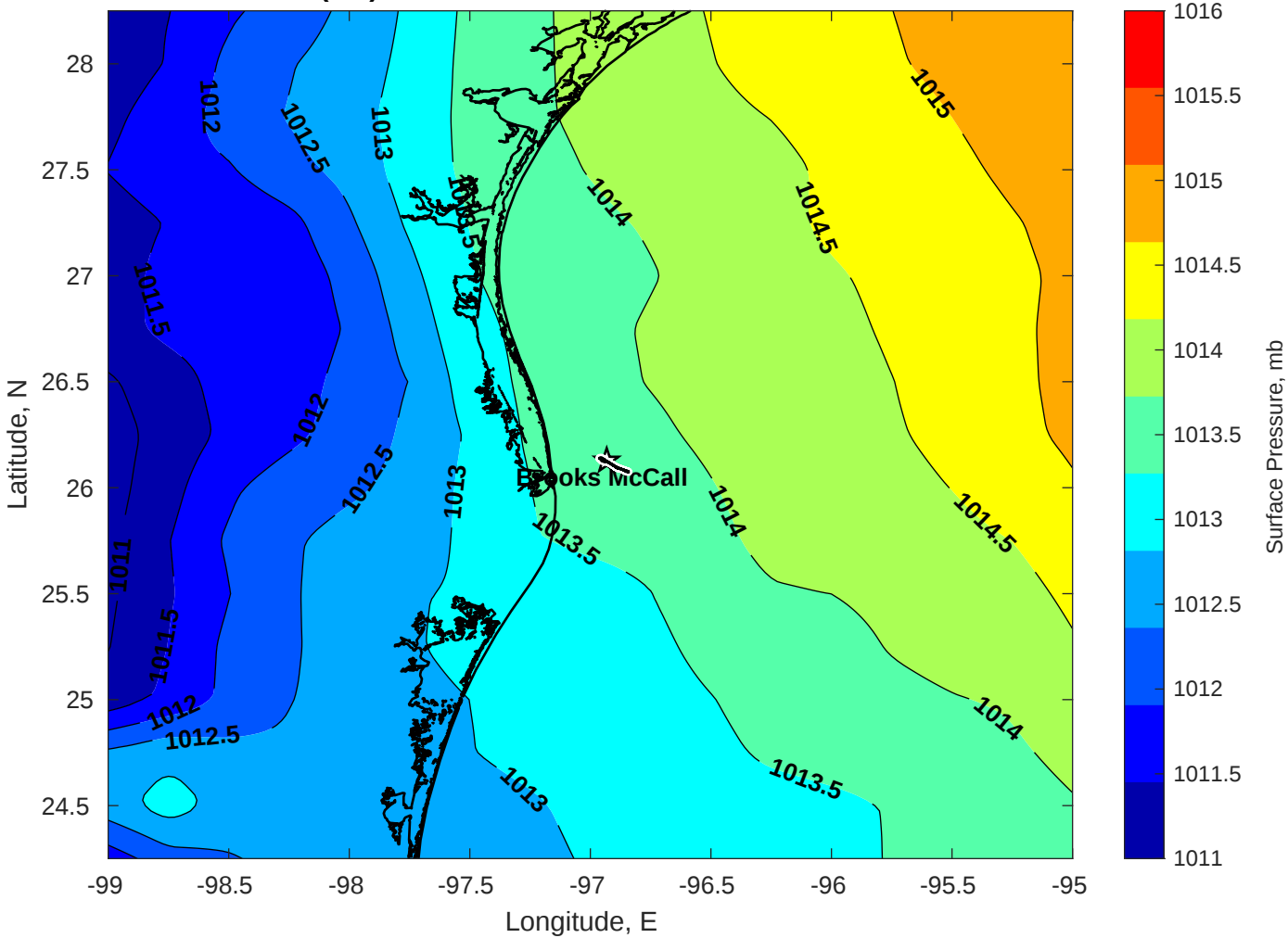
Surface Pressure (mb) for Brooks McCall at 30-Jun-2025 00:00:00
