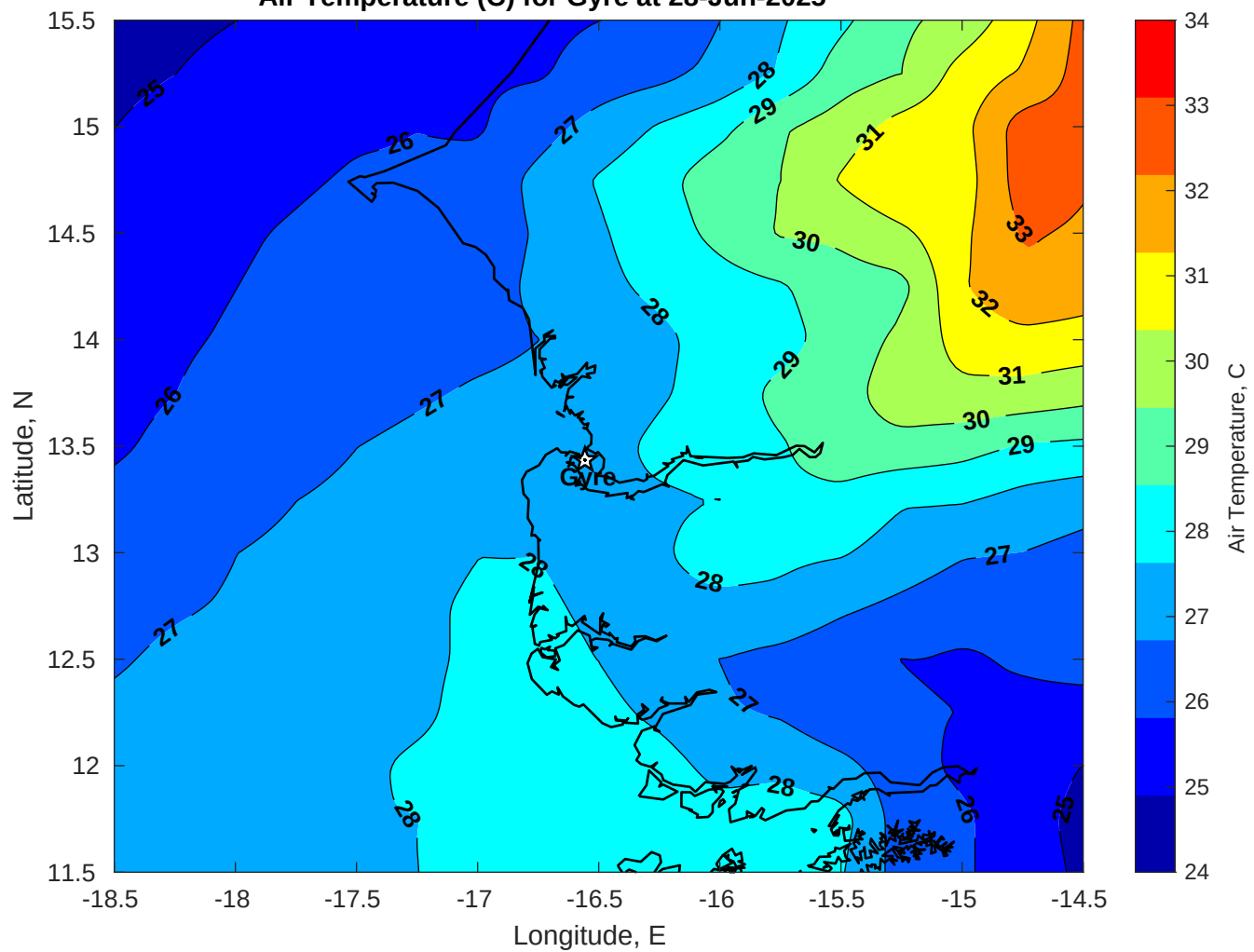
Air Temperature (C) for Gyre at 28-Jun-2025
