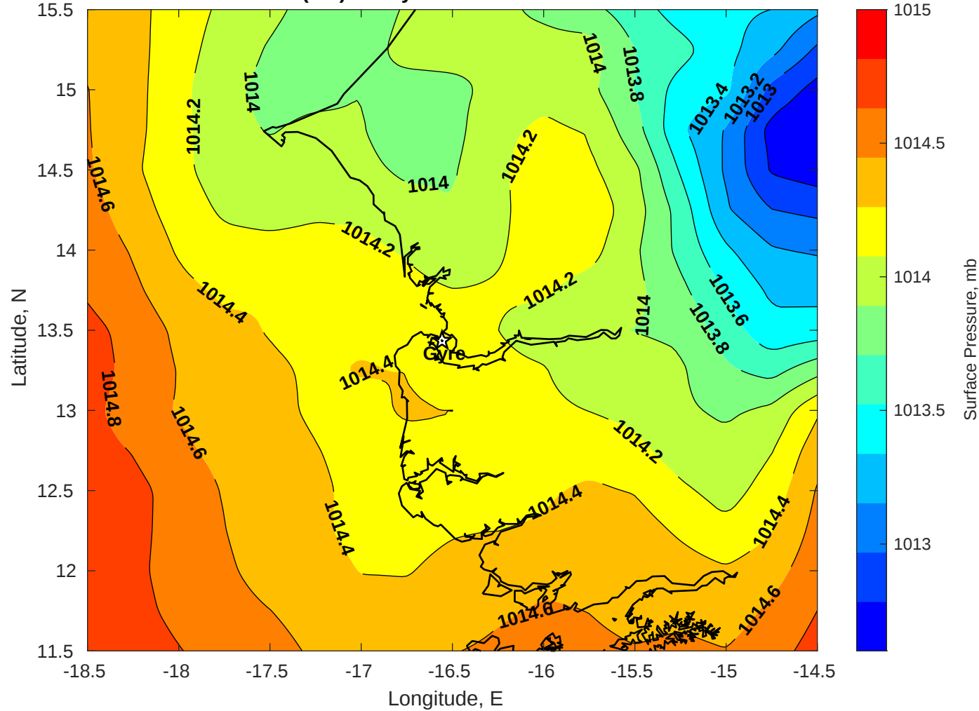
Surface Pressure (mb) for Gyre at 28-Jun-2025 00:00:00
