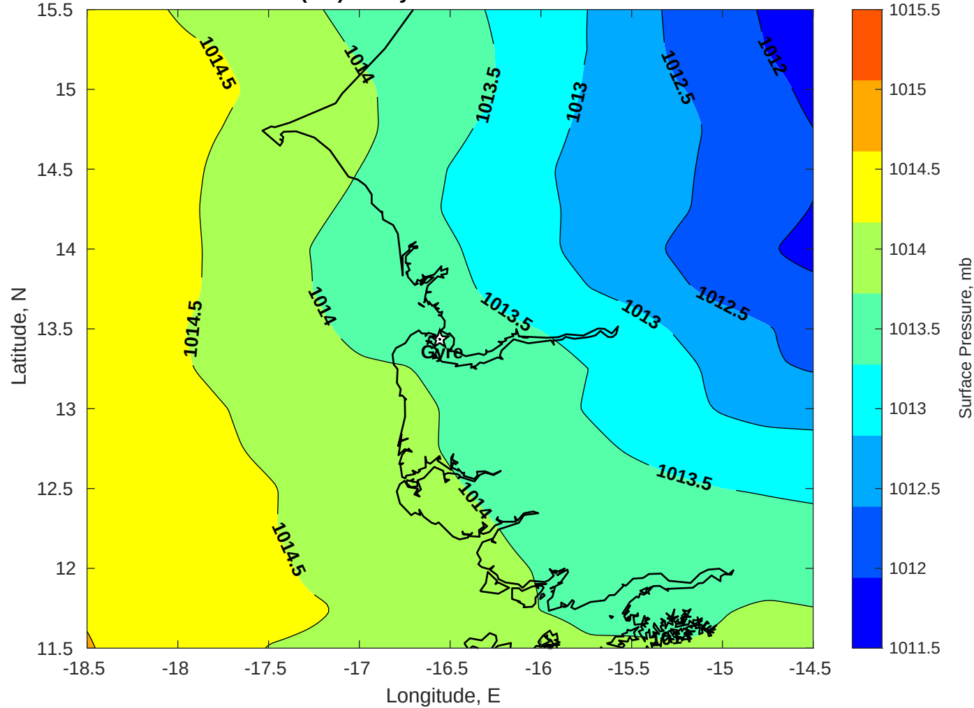
Surface Pressure (mb) for Gyre at 30-Jun-2025 00:00:00
