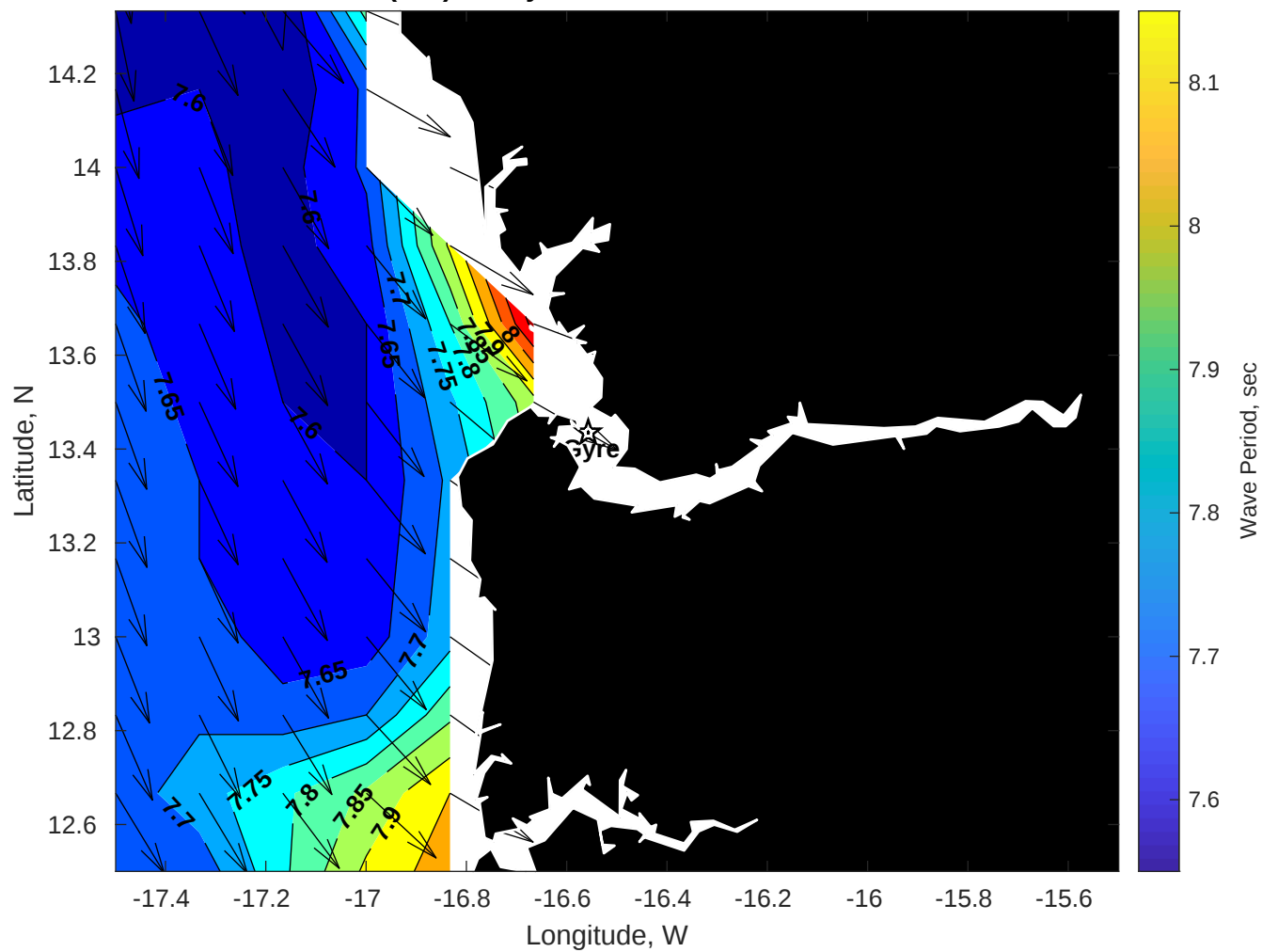
Wave Period (sec) for Gyre at 28-Jun-2025 09:00:00
