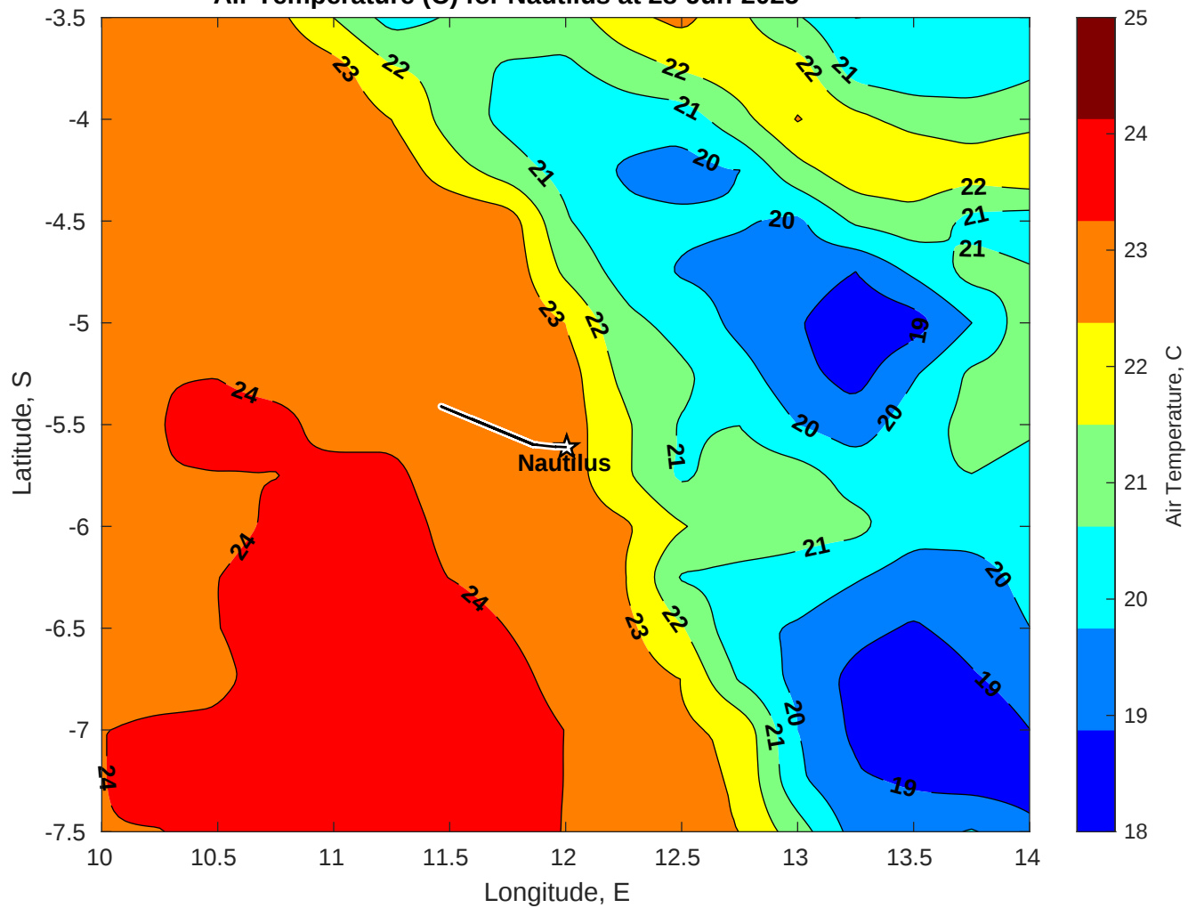
Air Temperature (C) for Nautilus at 28-Jun-2025
