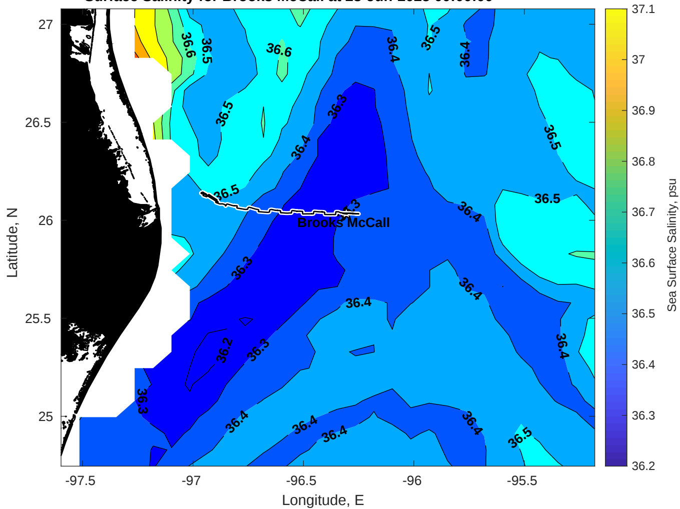
Surface Salinity for Brooks McCall at 28-Jun-2025 00:00:00
