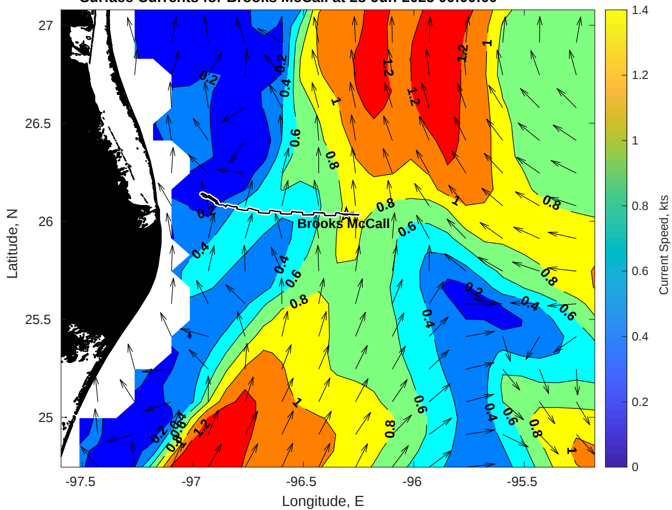
Surface Currents for Brooks McCall at 28-Jun-2025 00:00:00
