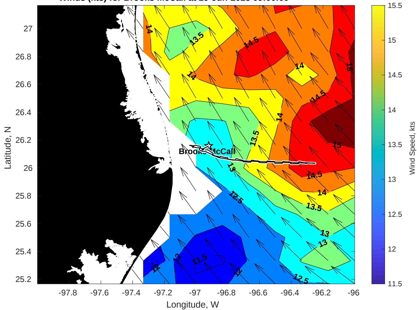
Winds (kts) for Brooks McCall at 29-Jun-2025 09:00:00
