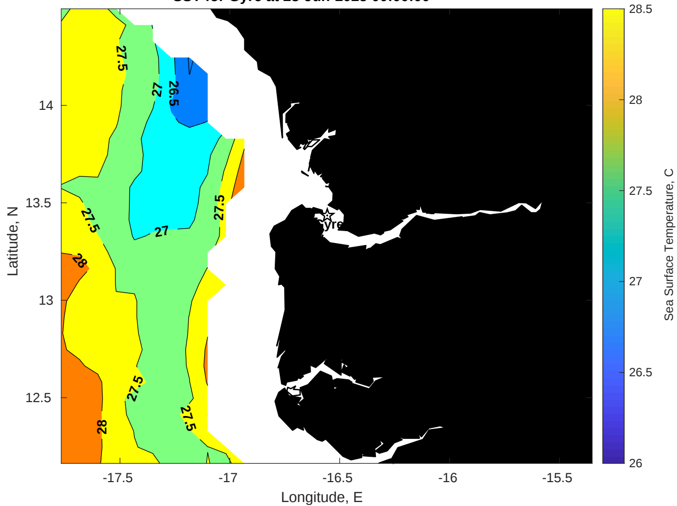
SST for Gyre at 28-Jun-2025 00:00:00
