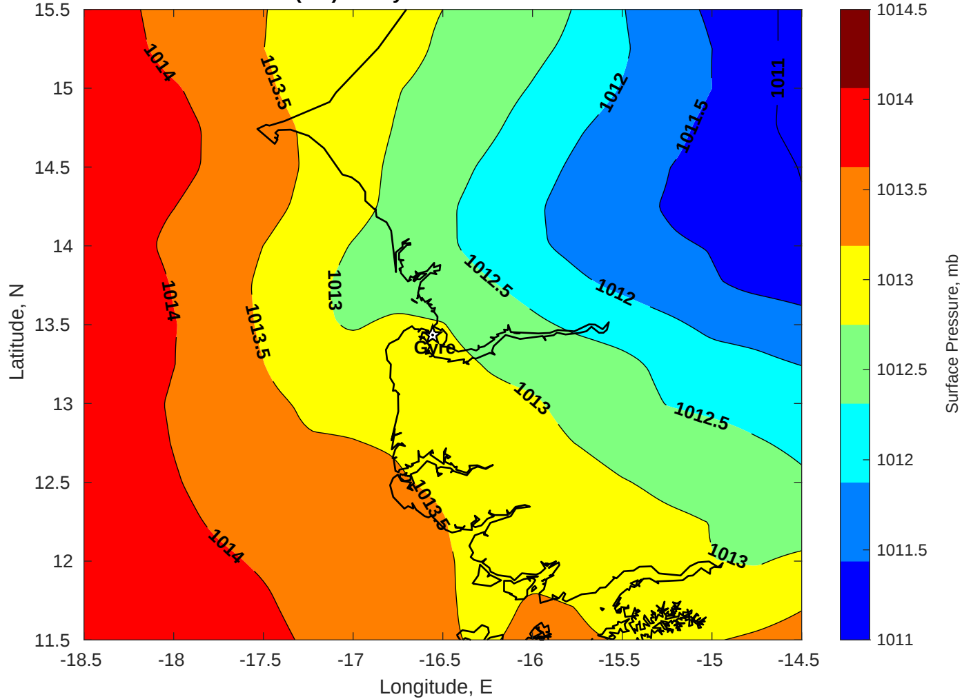
Surface Pressure (mb) for Gyre at 30-Jun-2025 00:00:00
