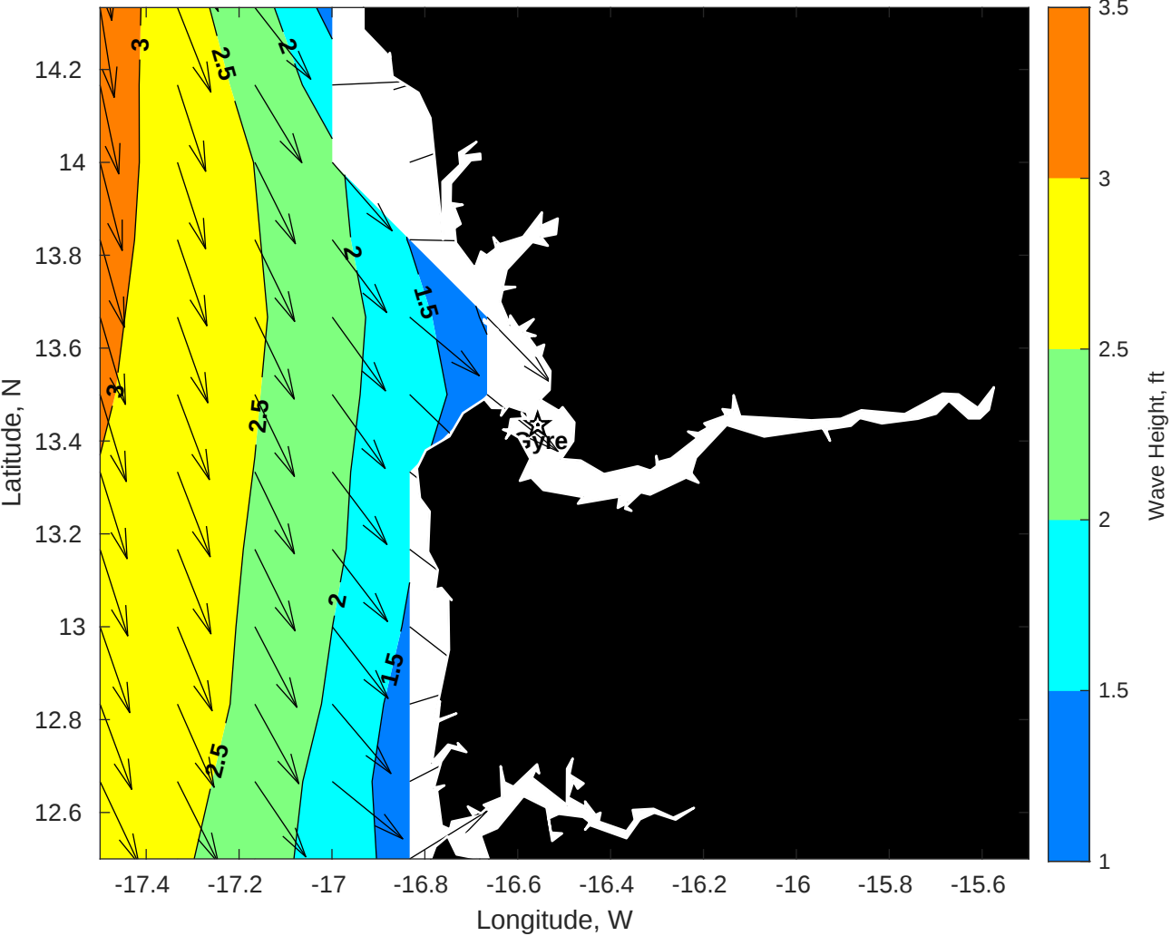
Wave Height (ft) for Gyre at 29-Jun-2025 09:00:00
