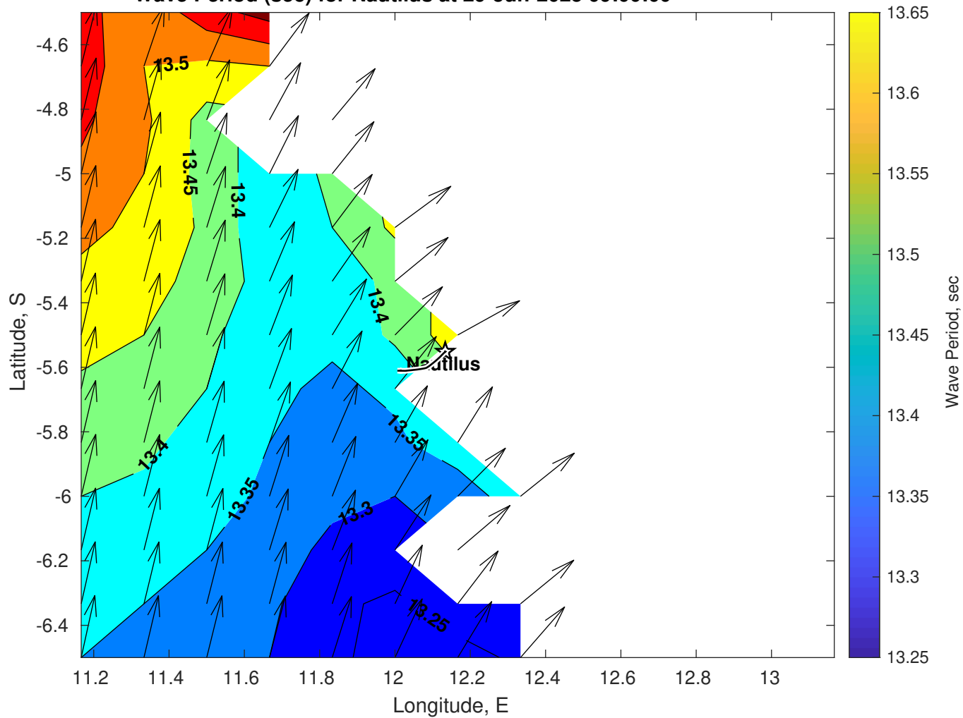
Wave Period (sec) for Nautilus at 29-Jun-2025 09:00:00
