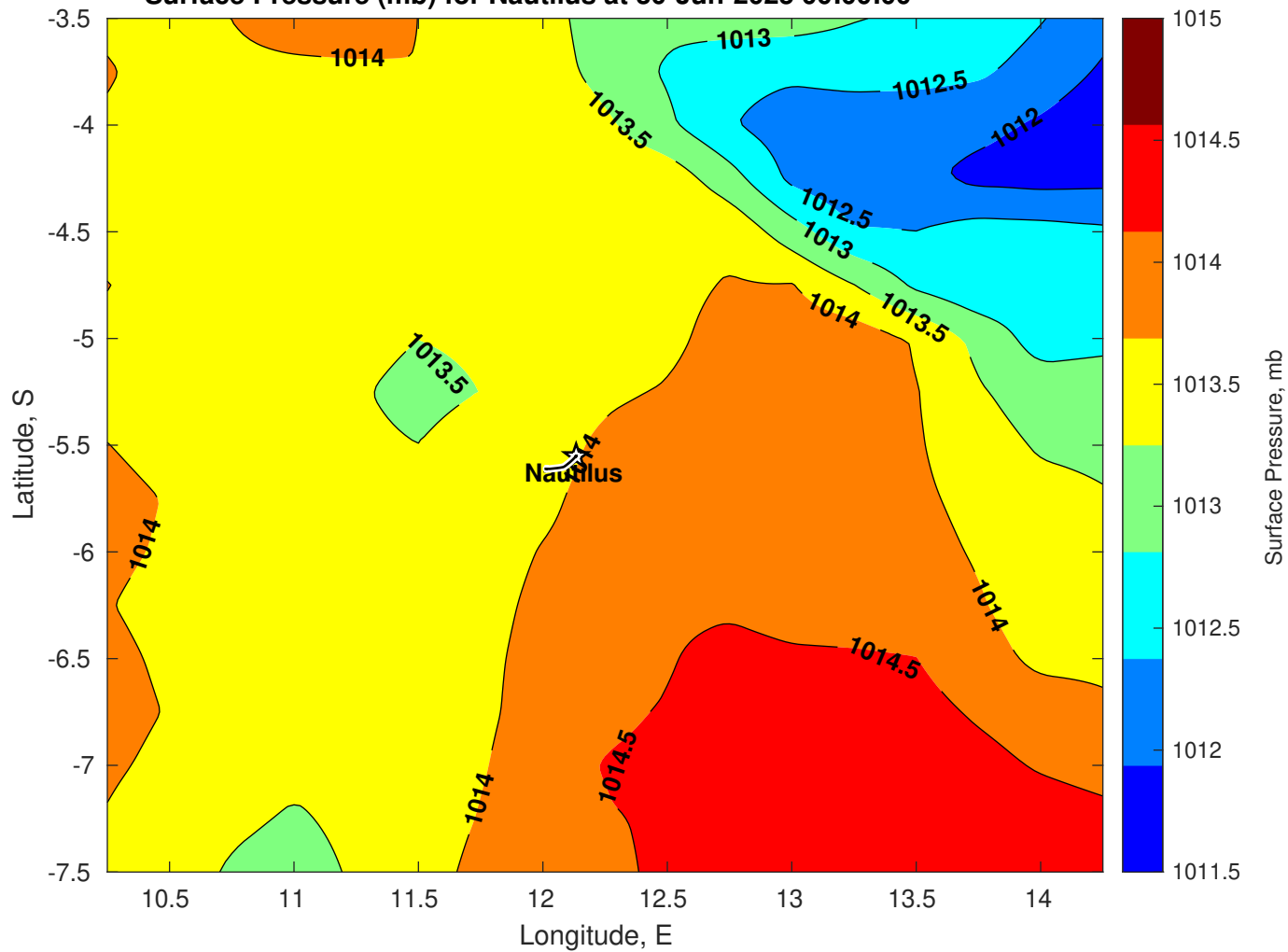
Surface Pressure (mb) for Nautilus at 30-Jun-2025 00:00:00
