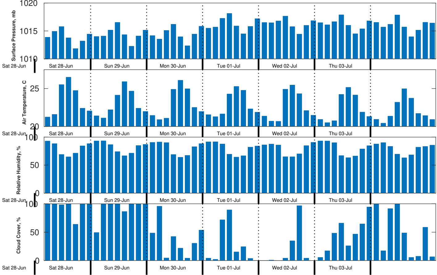
Met Forecast for Nautilus from 29-Jun-2025 00:00:00 to 06-Jul-2025 00:00:00
