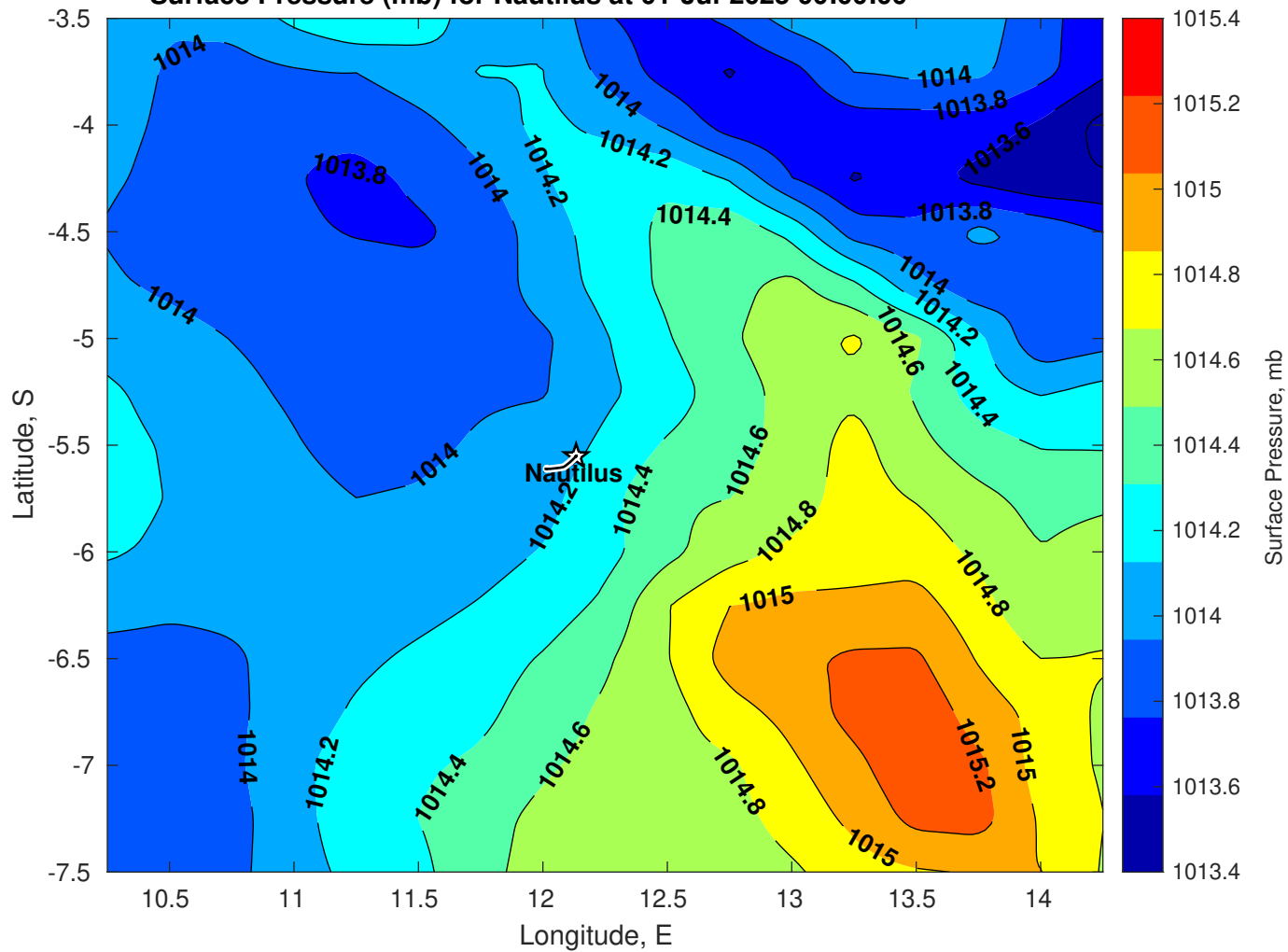
Surface Pressure (mb) for Nautilus at 01-Jul-2025 00:00:00
