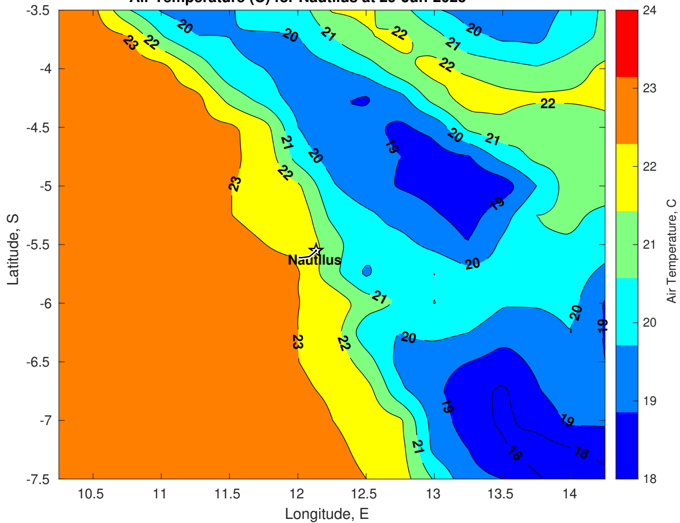
Air Temperature (C) for Nautilus at 29-Jun-2025
