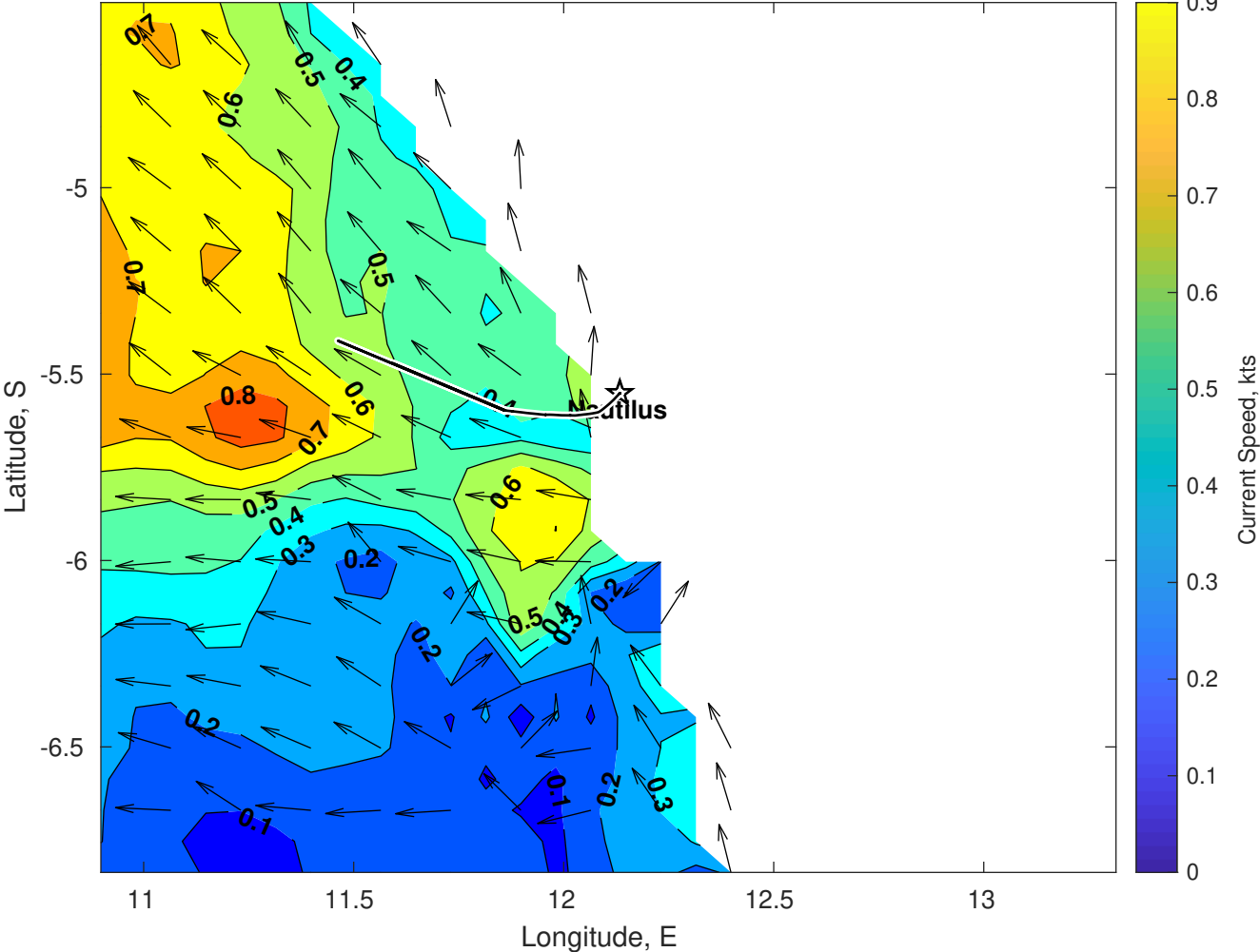
Surface Currents for Nautilus at 28-Jun-2025 00:00:00
