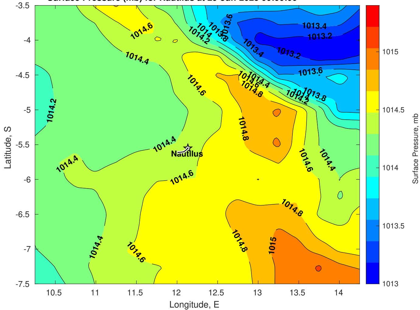
Surface Pressure (mb) for Nautilus at 29-Jun-2025 00:00:00
