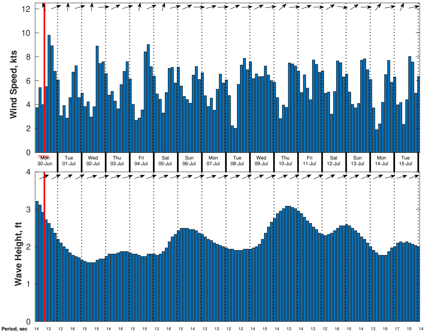
Wind & Wave Forecast for Nautilus from 29-Jun-2025 02:00:00 to 15-Jul-2025 02:00:00
