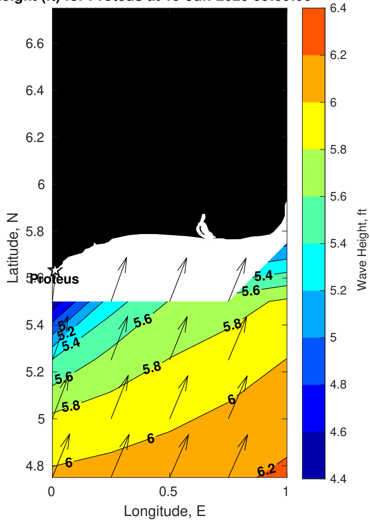
Wave Height (ft) for Proteus at 19-Jun-2025 09:00:00
