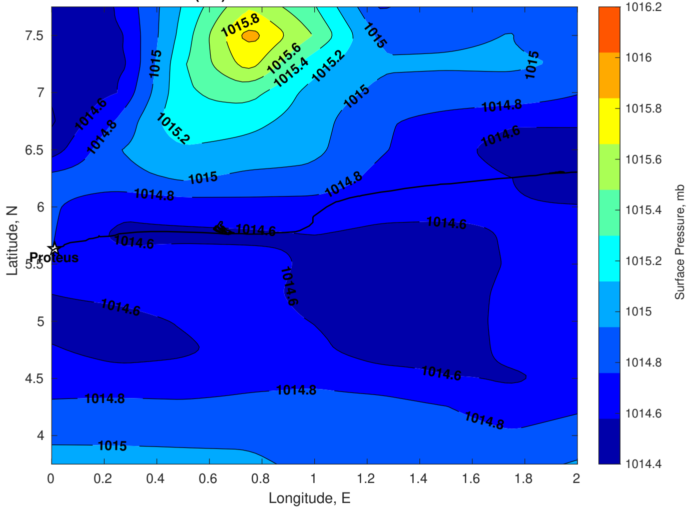
Surface Pressure (mb) for Proteus at 20-Jun-2025 00:00:00
