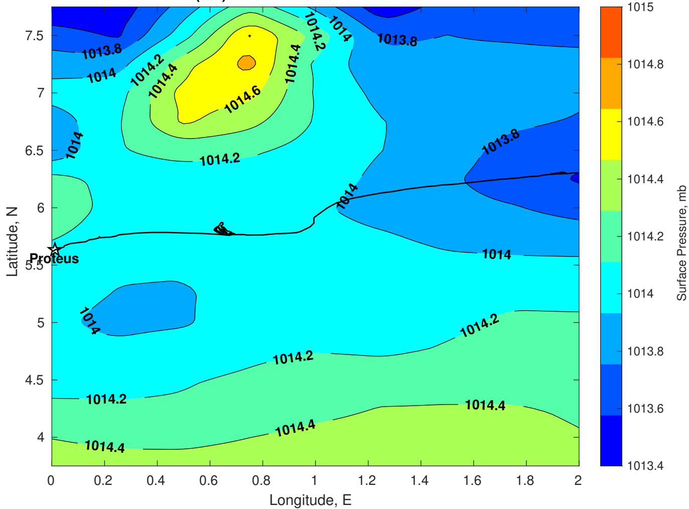
Surface Pressure (mb) for Proteus at 21-Jun-2025 00:00:00
