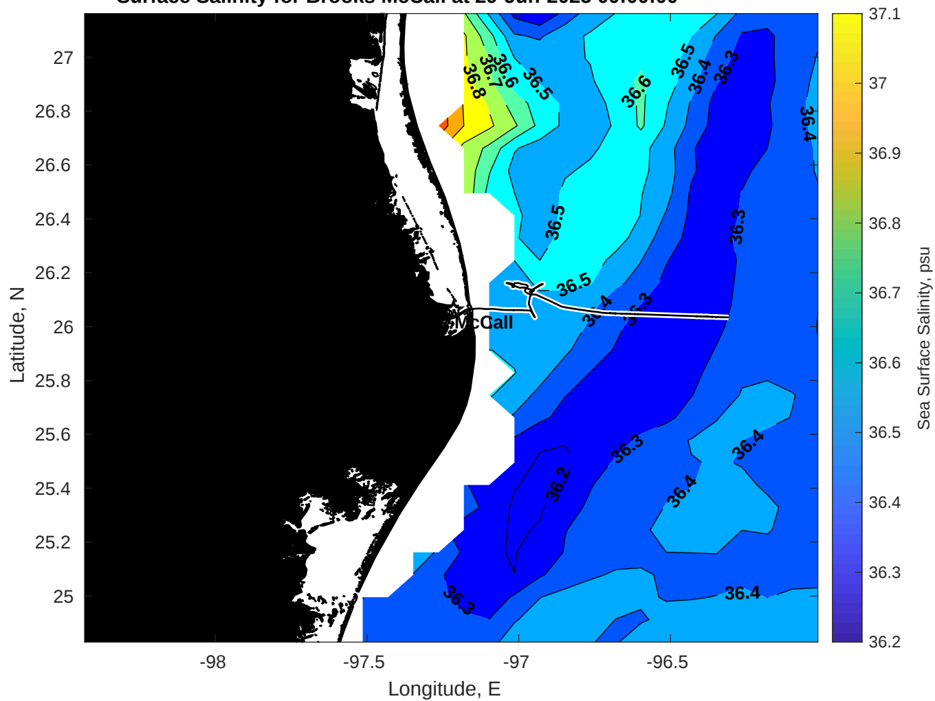
Surface Salinity for Brooks McCall at 29-Jun-2025 00:00:00
