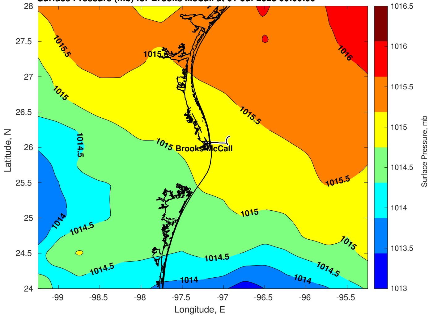
Surface Pressure (mb) for Brooks McCall at 01-Jul-2025 00:00:00
