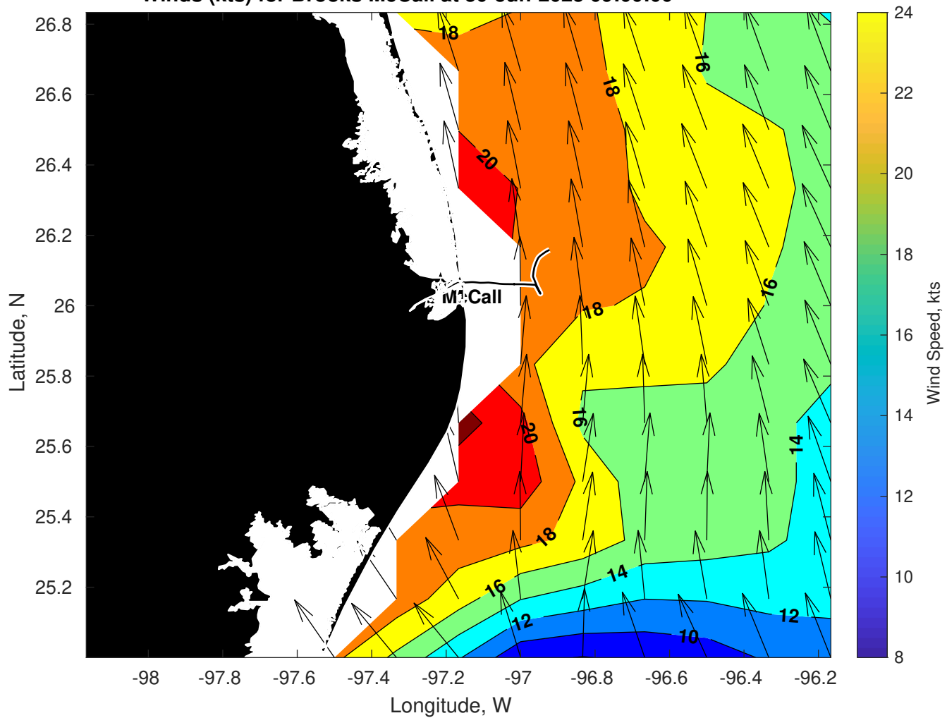
Winds (kts) for Brooks McCall at 30-Jun-2025 09:00:00
