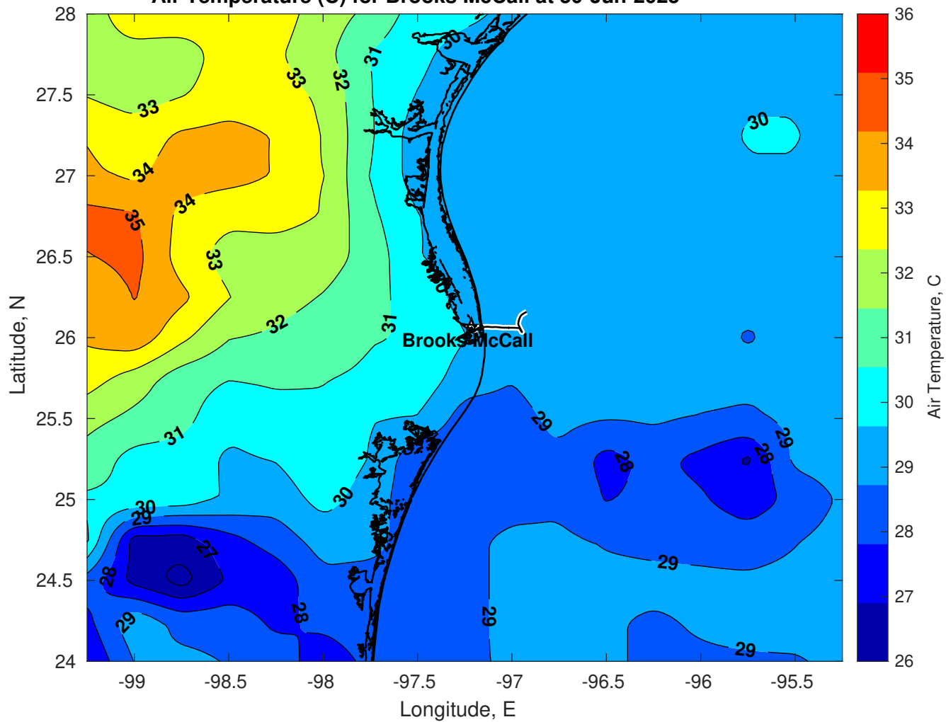
Air Temperature (C) for Brooks McCall at 30-Jun-2025
