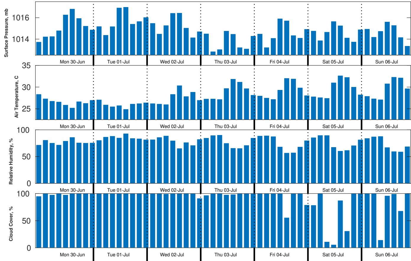
Met Forecast for Brooks McCall from 30-Jun-2025 00:00:00 to 07-Jul-2025 00:00:00
