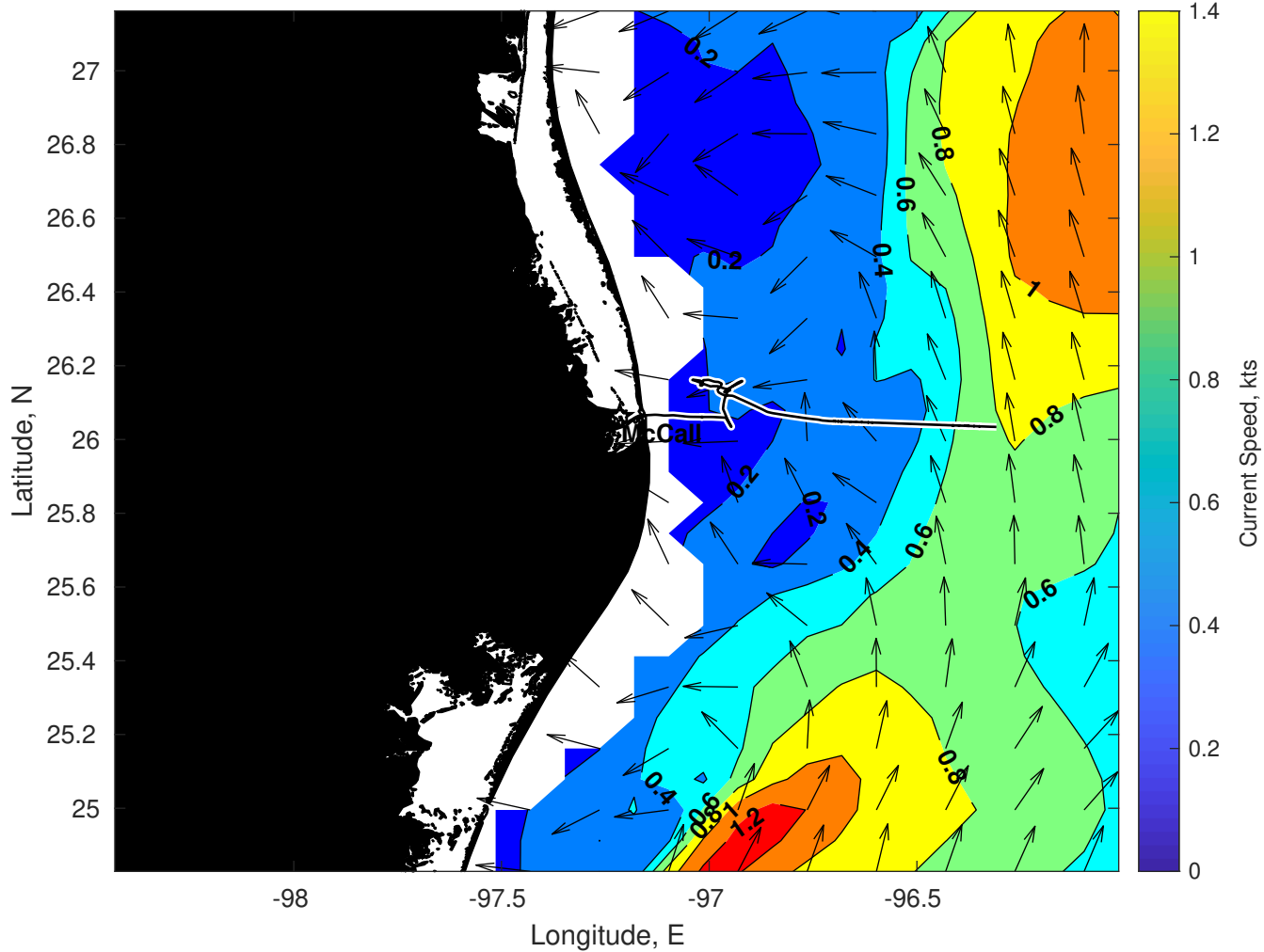
Surface Currents for Brooks McCall at 29-Jun-2025 00:00:00
