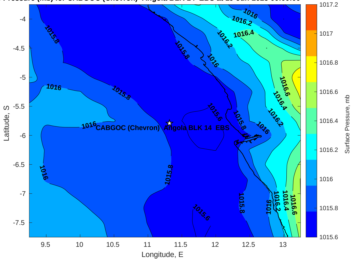
Surface Pressure (mb) for CABGOC (Chevron) Angola BLK 14 EBS at 19-Jun-2025 00:00:00
