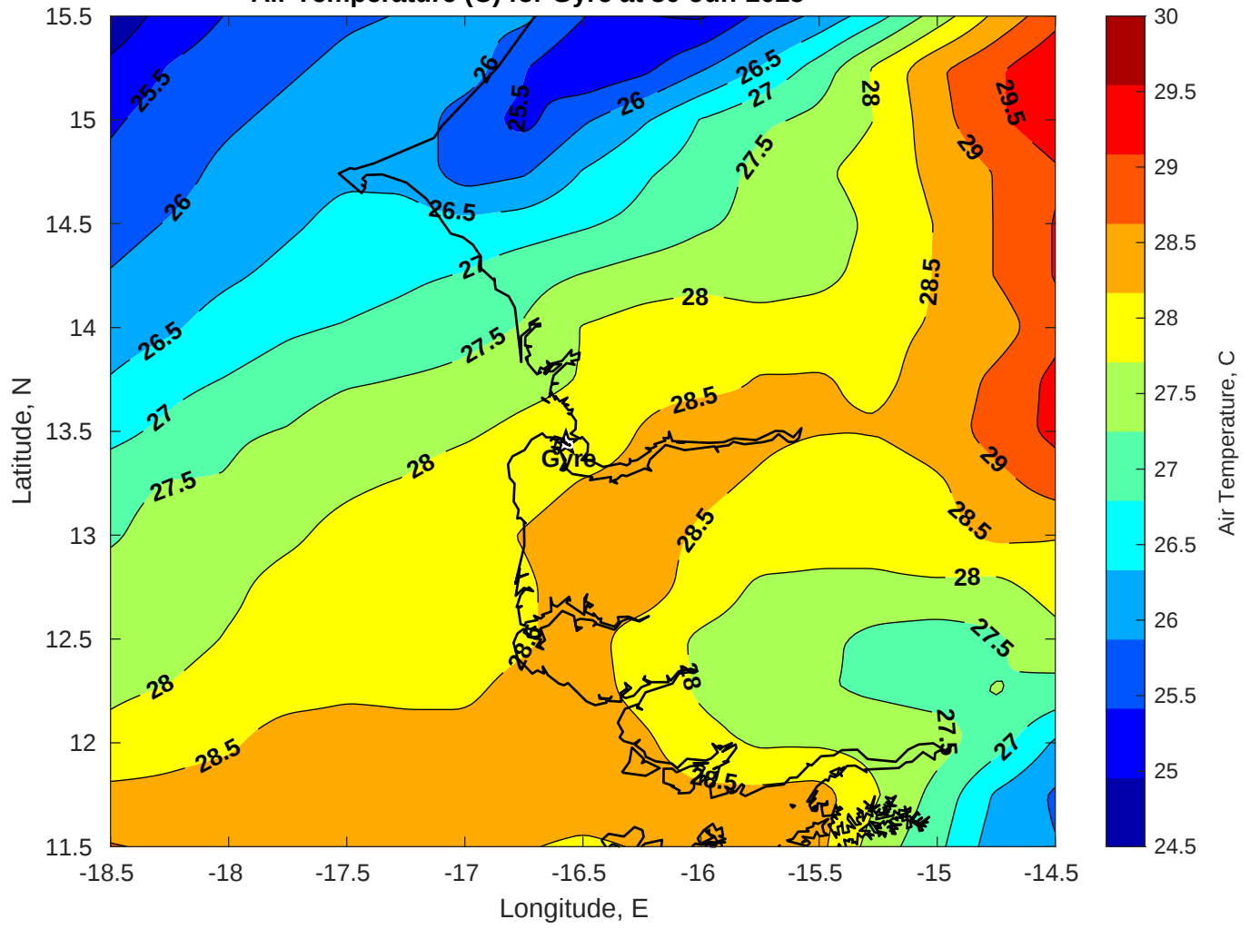
Air Temperature (C) for Gyre at 30-Jun-2025
